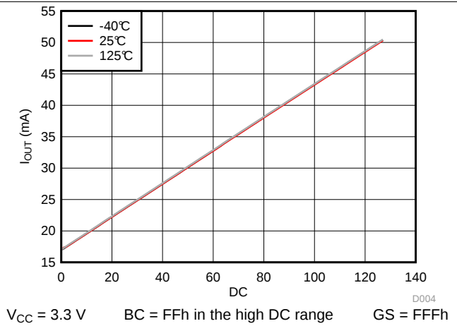
图 18. I_{OUT} vs Dot Correction at Different Ambient Temperatures
