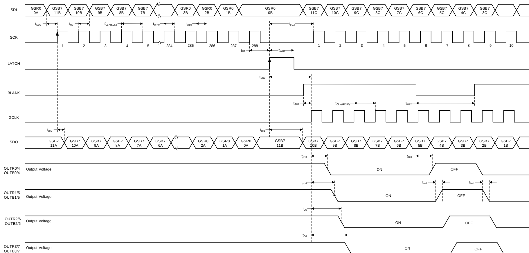
图 1. Grayscale Data (GS) Write
