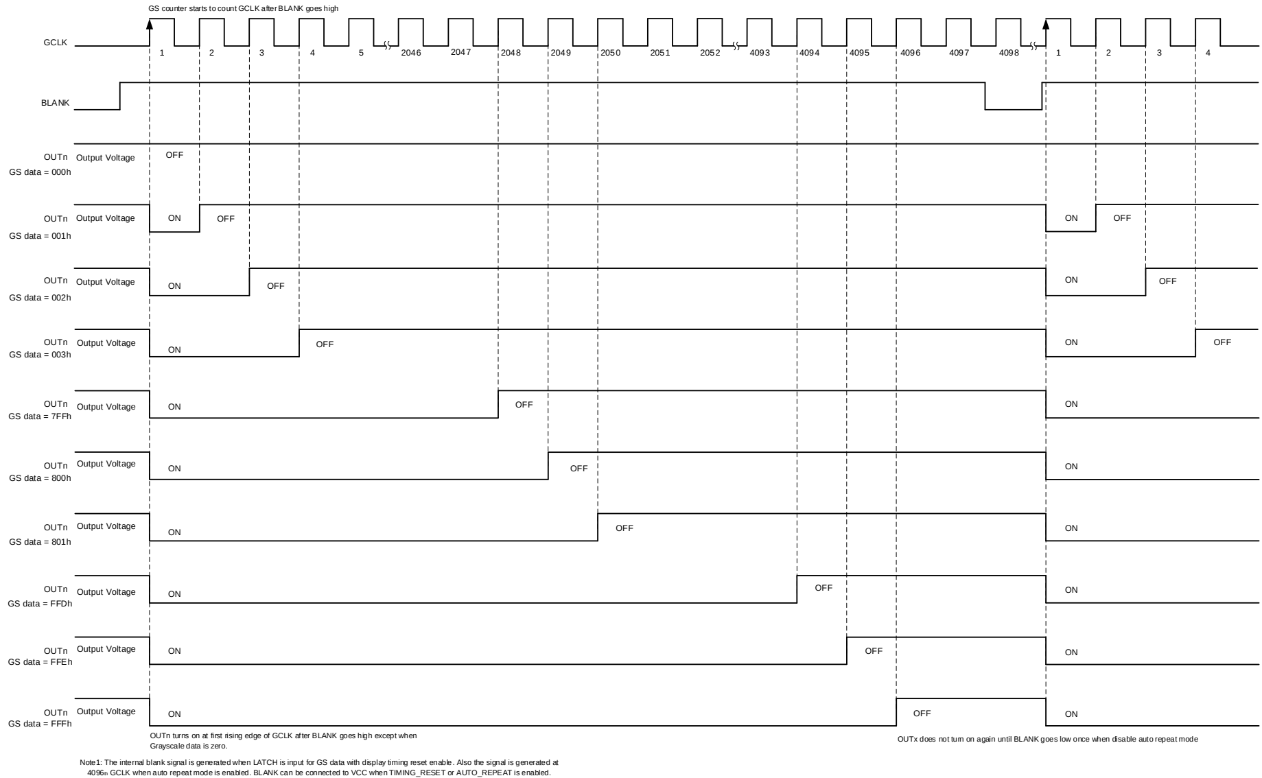
图 11. 12-Bit Mode PWM Counter Without Auto-Repeat Mode
