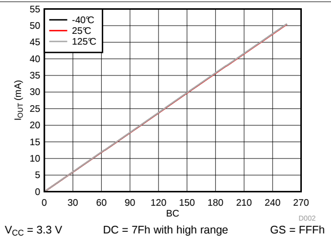
图 20. I_{OUT} vs Brightness Control at Different Ambient Temperatures
