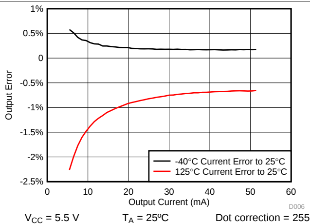
图 9. Output Temperature Error vs Output Current
