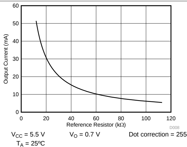
图 11. Output Current vs Reference Resistor
