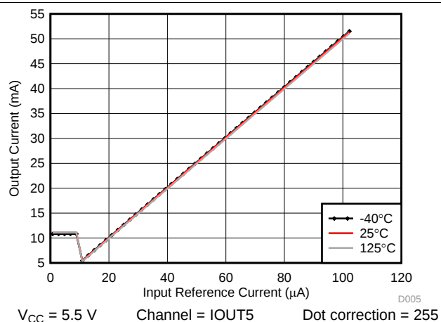
图 6. Output Current vs Reference Current
