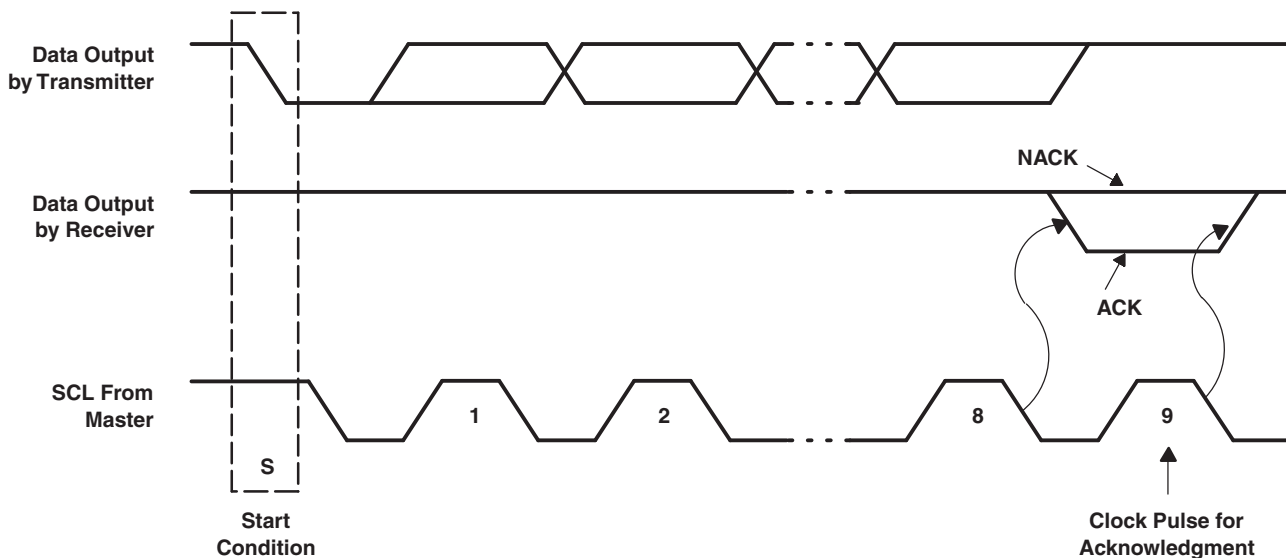
Figure 12. Acknowledge/Not Acknowledge on I²C Bus
