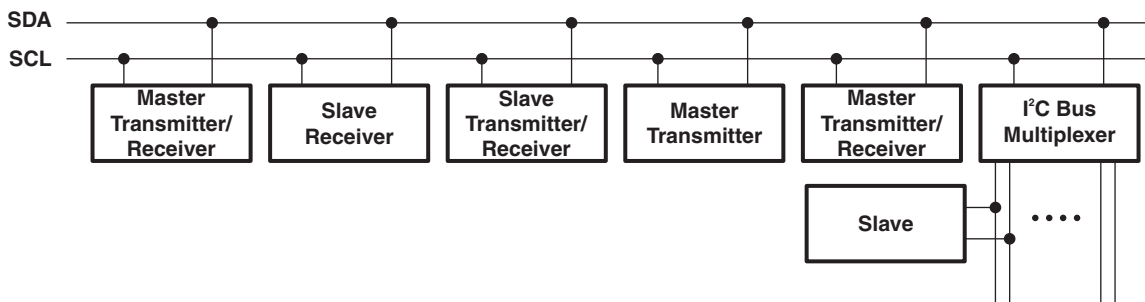
Figure 18. System Configuration
