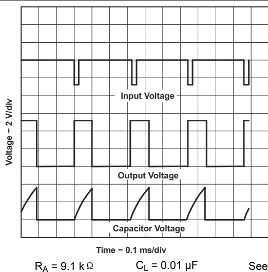
图 6-3. Typical Monostable Waveforms
