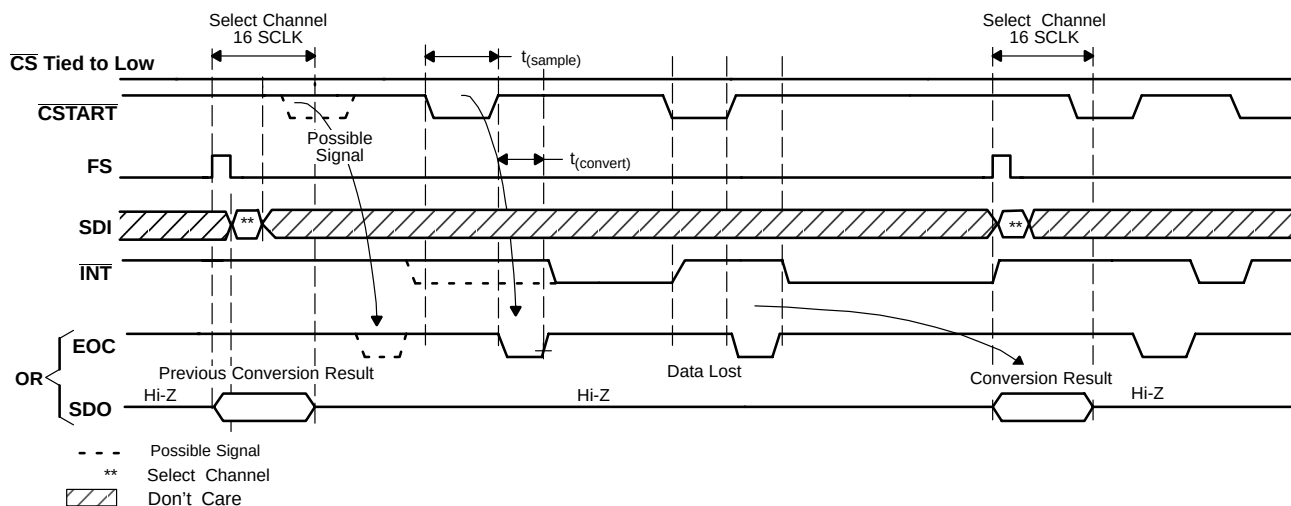
Figure 14. Mode 00, \overline{CSTART} Triggers Sampling/Conversion, FS Initiates Select
