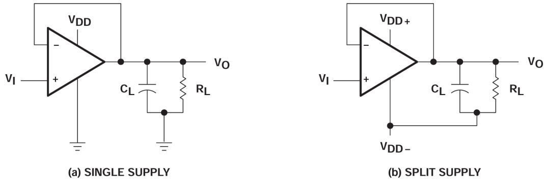
Figure 6-1. Unity-Gain Amplifier
