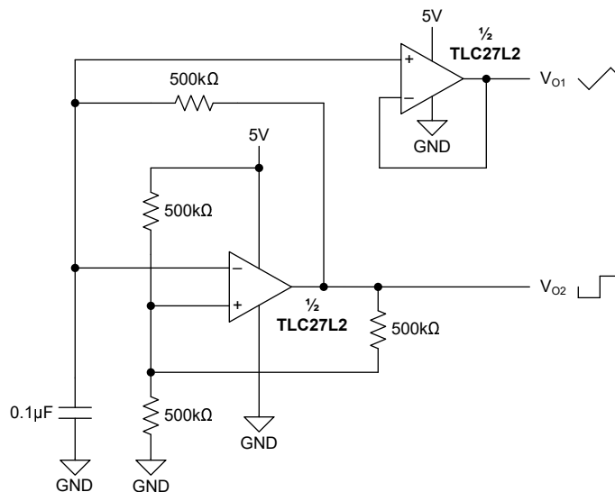
Figure 7-9. Multivibrator
