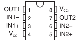
TL972...D OR PW PACKAGE (TOP VIEW)
