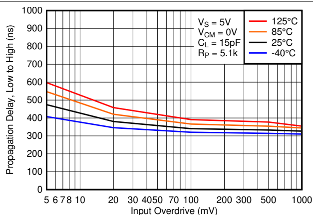
图 5-26. Low to High Propagation Delay vs. Input Overdrive Voltage, 5V
