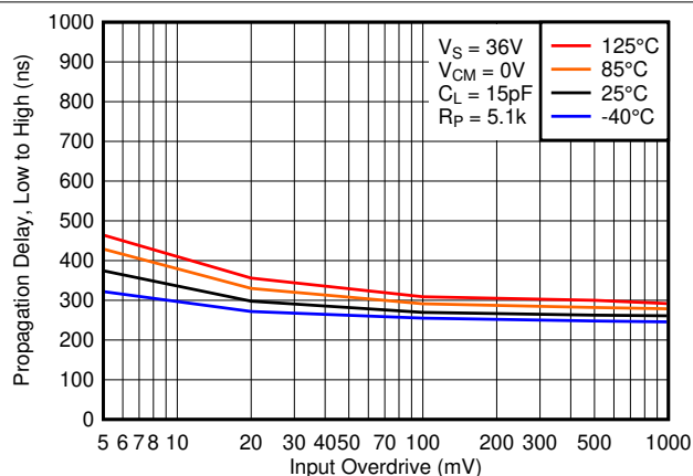
图 5-30. Low to High Propagation Delay vs. Input Overdrive Voltage, 36V
