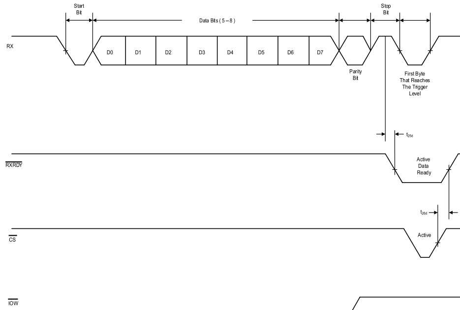
图 13. Receive Timing in FIFO Mode ( \overline{\text{IOW}} Only Mode, \text{MODE} = \text{GND} )
