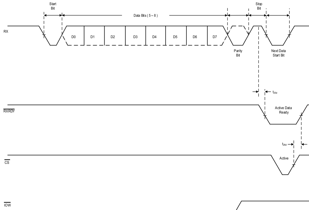
图 11. Receive Ready Timing in Non-FIFO Mode ( \overline{\text{IOW}} Only Mode, MODE = GND)
