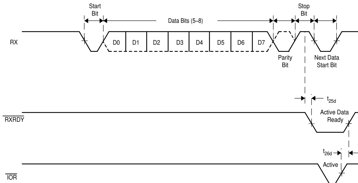
图 10. Receive Ready Timing in Non-FIFO Mode ( \overline{\text{IOR}} and \overline{\text{IOW}} Mode, MODE = VCC)
