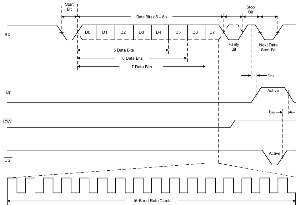
图 9. Receive Timing ( \overline{\text{IOW}} Only Mode, MODE = GND)
