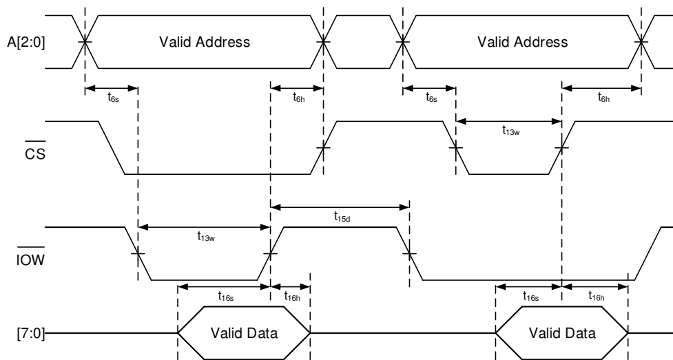
图 2. General Write Timing ( \overline{IOW} and \overline{IOW} Mode, MODE = VCC)
