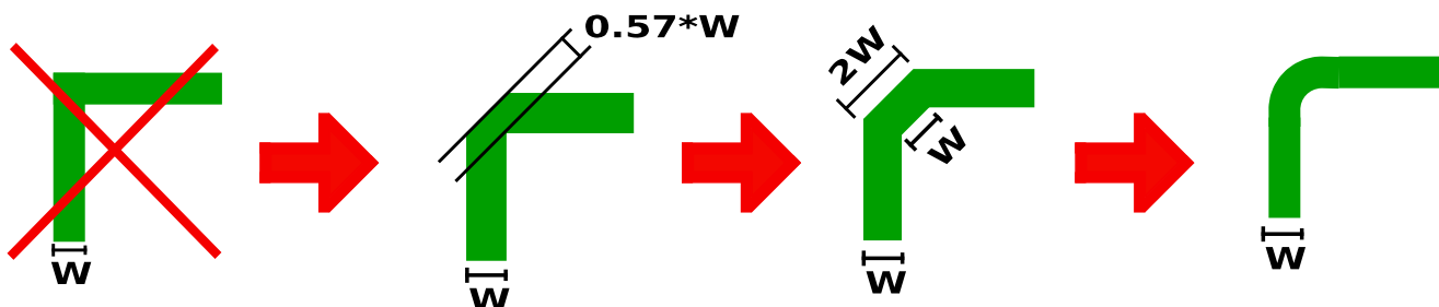
图 46. Layout Do's and Don'ts
