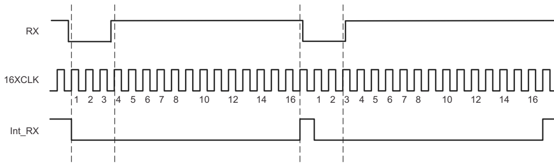
图 39. Timing Causing 1-Clock-Wide Pulse Between Consecutive Ones
