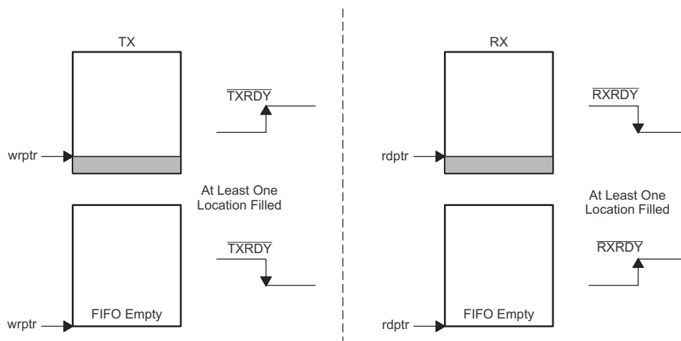
图 28. \overline{\text{TXRDY}} and \overline{\text{RXRDY}} in DMA Mode 0 or FIFO Disable
