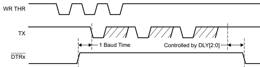
图 31. DTRx and Transmit Data Relationship
