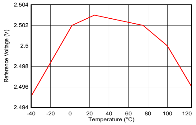
图 5-18. Reference Voltage vs Temperature
