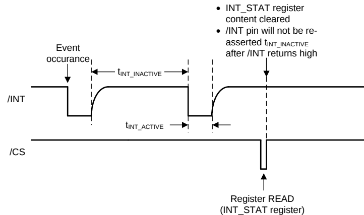
图 18. Dynamic \overline{INT} Assertion Scheme With INT_STAT Register Read During t_{INT\_INACTIVE}
