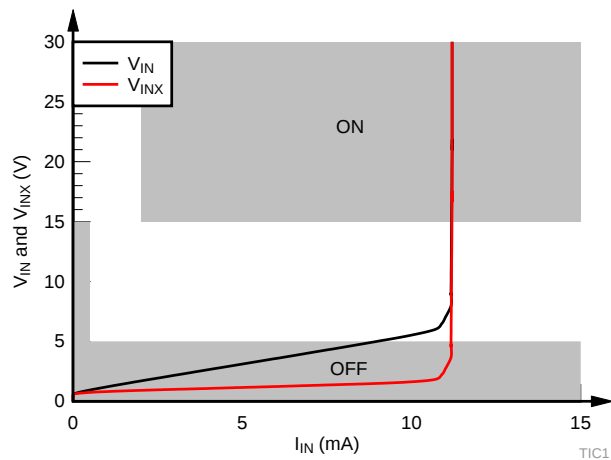
图 84. Type-1 Switch with 400- \Omega Input Resistor
