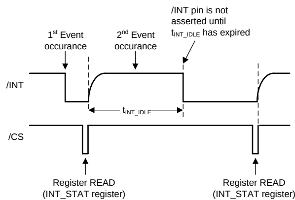
图 19. \overline{INT} Assertion Scheme With t_{INT\_IDLE}
