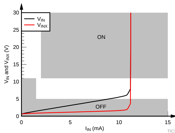
图 86. Type-3 Switch with 400- \Omega Input Resistor
