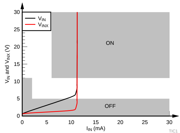
图 85. Type-2 Switch with 400- \Omega Input Resistor
