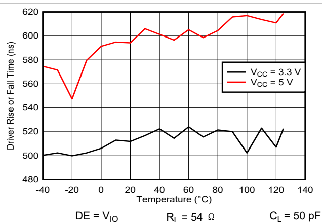
图 5-5. THVD2410V 250kbps Driver rise or fall time vs Temperature
