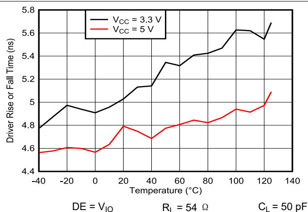
图 5-11. THVD2450V 50Mbps Driver rise or fall time vs Temperature
