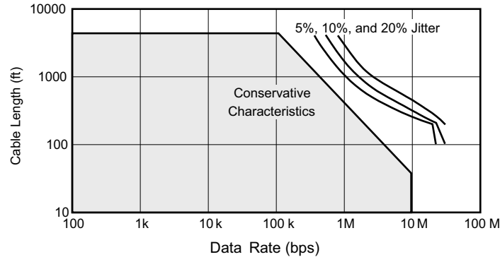
图 8-3. Cable Length vs Data Rate Characteristic
