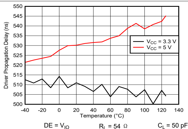
图 5-6. THVD2410V 250kbps Driver propagation delay vs Temperature
