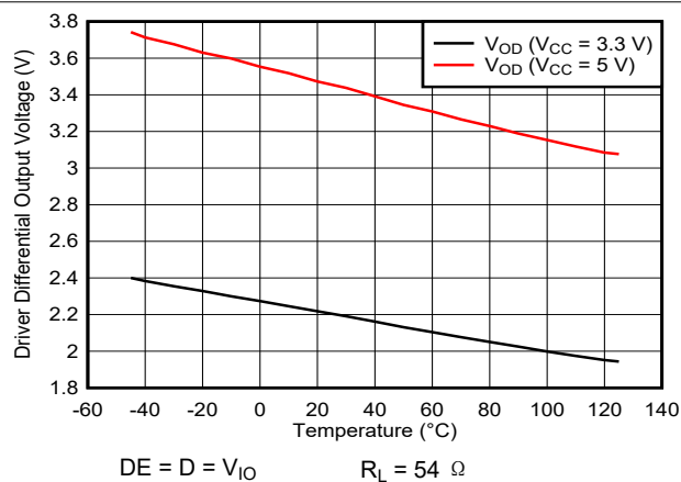
图 5-4. Driver differential output voltage vs Temperature
