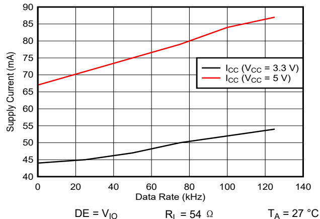
图 5-14. THVD2410V Supply Current vs Signal Rate
