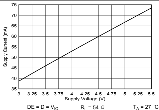
图 5-3. Supply Current vs Supply Voltage
