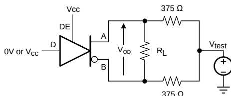
图 11. Measurement of Driver Differential Output Voltage With Common-Mode Load
