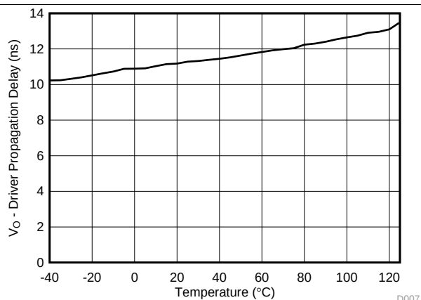
图 7. THVD1550 Driver Propagation Delay vs Temperature
