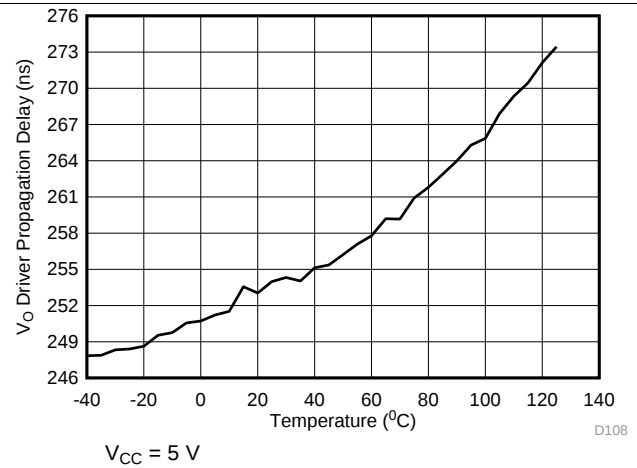
图 15. Driver Propagation Delay vs Temperature
