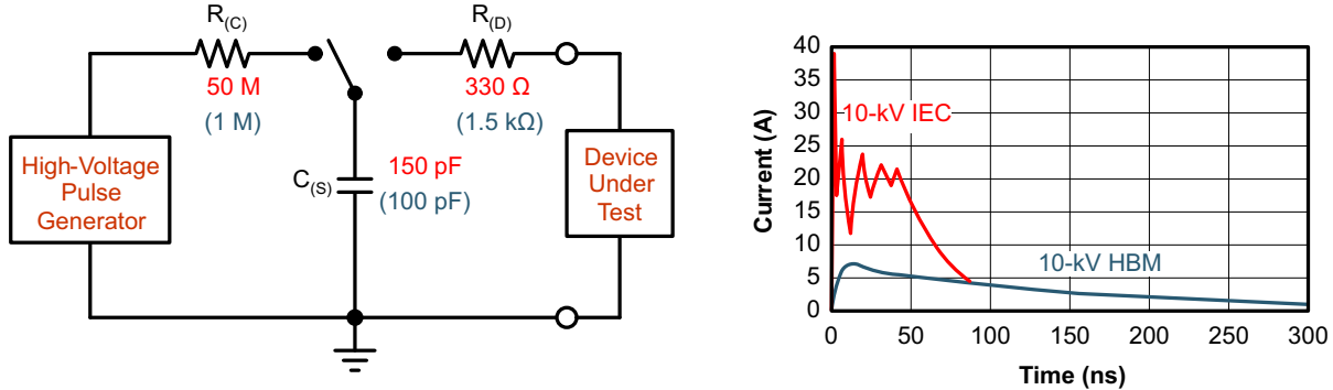
图 8-2. HBM and IEC ESD Models and Currents in Comparison (HBM Values in Parenthesis)
