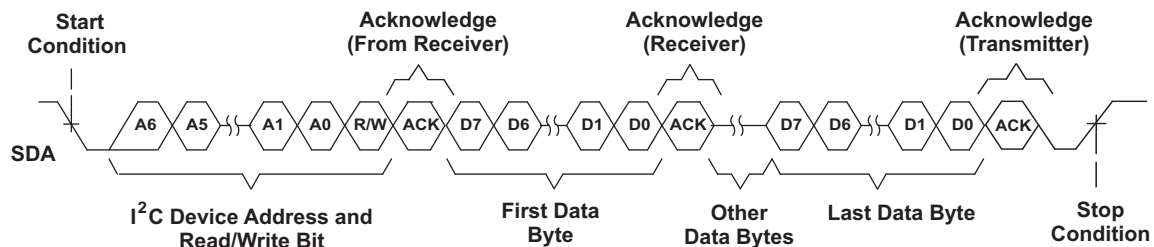
Figure 76. Multiple Byte Write Transfer
