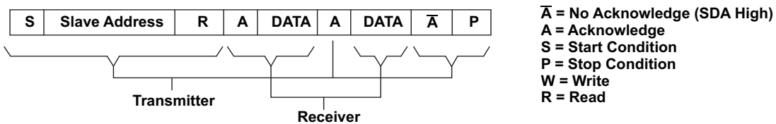
Figure 77. I²C Read Cycle
