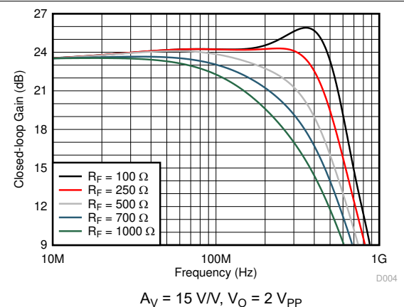
图 5-6. Small-Signal Frequency Response vs R_F
