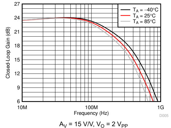
图 5-4. Small-Signal Frequency Response vs Temperature
