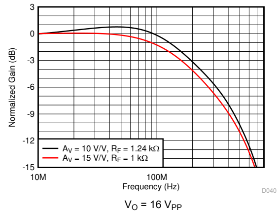
图 5-2. Large-Signal Frequency Response
