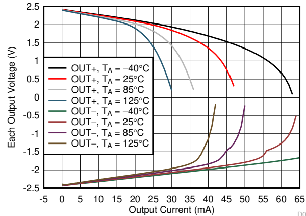
图 7-28. ±Maximum Output Voltage vs Output Current and Temperature
