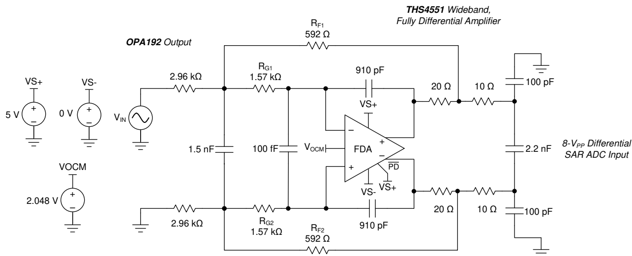
图 10-11. Example 100-kHz Butterworth Filter
