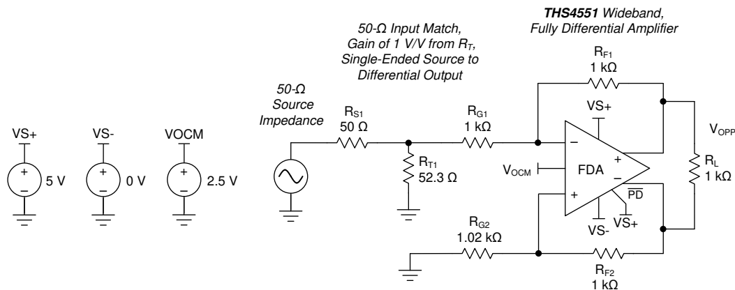
Figure 9-9. DC-Coupled Gain of 1 with R_F = 1\text{ k}\Omega and Single-to-Differential Matched Input 50\text{-}\Omega Impedance
