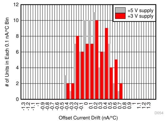
图 6-52. Input Offset Current Over Temperature
