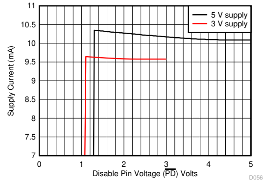
图 6-56. Supply Current vs \overline{\text{PD}} Voltage
