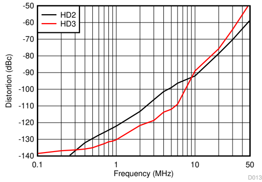
图 6-13. Harmonic Distortion Over Frequency
