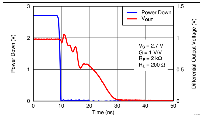
Figure 22. Turn-Off Time
