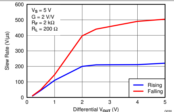
Figure 38. Single-Ended Slew Rate vs V_{OUT} Step
