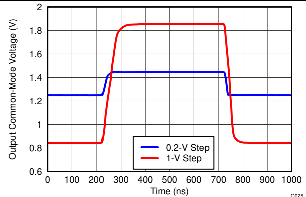
Figure 27. V_{OCM} Large and Small-Signal Pulse Response
