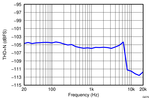
Figure 87 shows the THD+N vs Frequency with no weighting and Figure 88 shows an FFT with 1 kHz input tone. Input signal to the PCM4204 for these tests is -0.5 dBFS. Table 6 summarizes results of testing using the THS4531 + PCM4204 versus typical Data Sheet performance, and show it make an excellent drive amplifier for this ADC.
