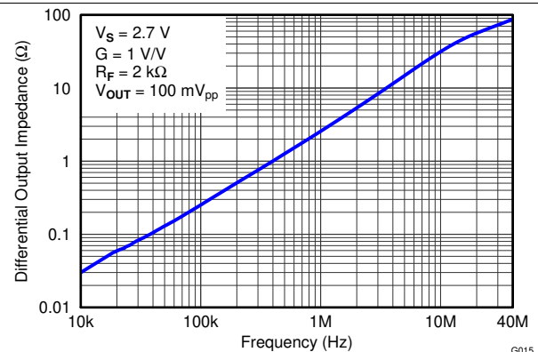
Figure 17. Main Amplifier Differential Output Impedance vs Frequency
