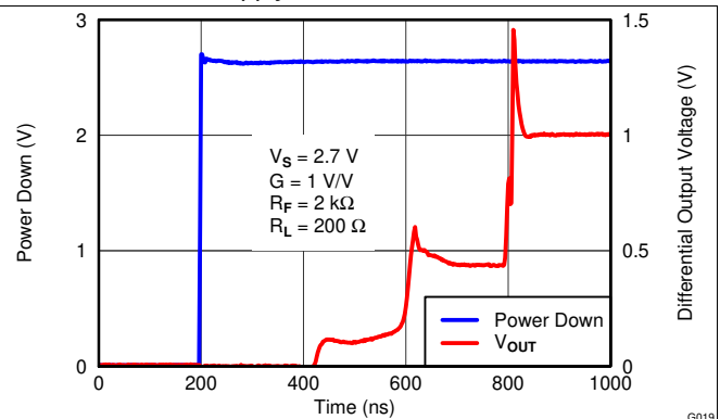
Figure 21. Turn-On Time
