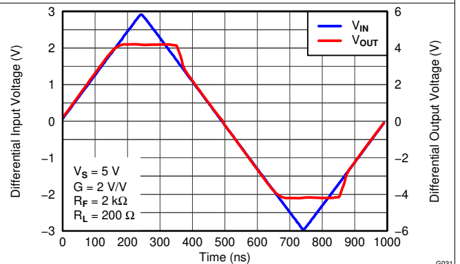
Figure 40. Overdrive Recovery
