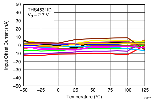
Figure 31. Input Offset Current vs Temperature
