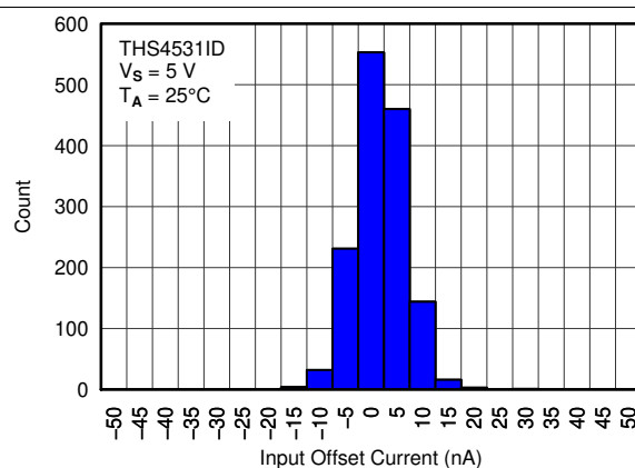
Figure 62. Input Offset Current Histogram
