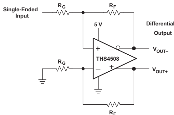
Figure 50. Single-Ended Input to Differential Output Amplifier
