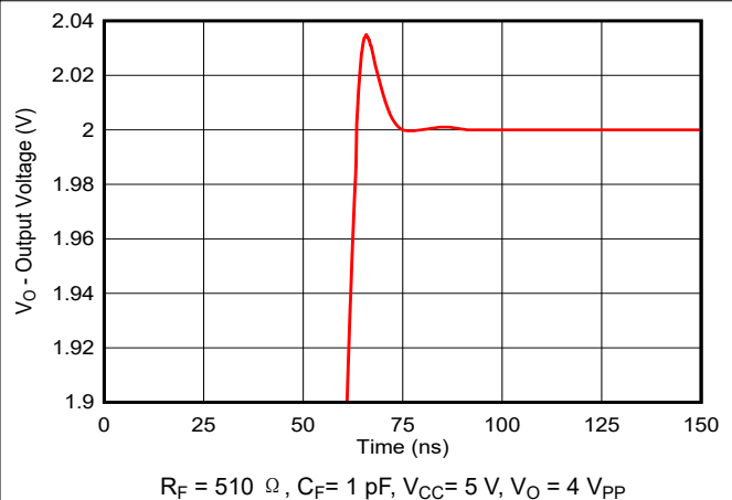
图 7-12. Settling Time
