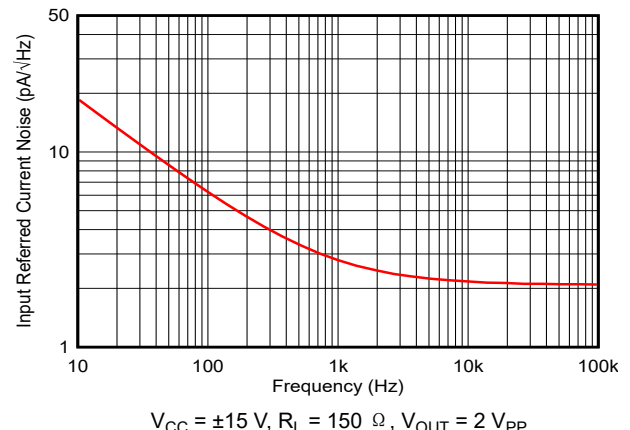
图 5-12. Input-Referred Current Noise vs Frequency
