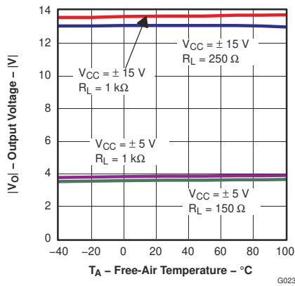
图 5-52. Output Voltage vs Free-air Temperature
