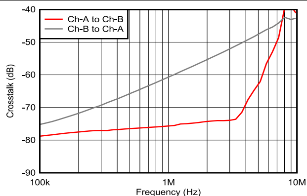
图 5-20. Crosstalk vs Frequency
