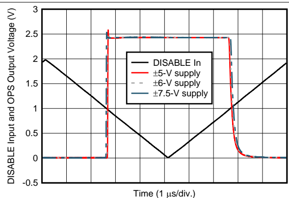
Figure 58. OPS Reverse Feedthrough in Disable
