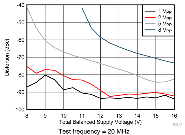
Figure 12. HD3 vs Supply Voltage
