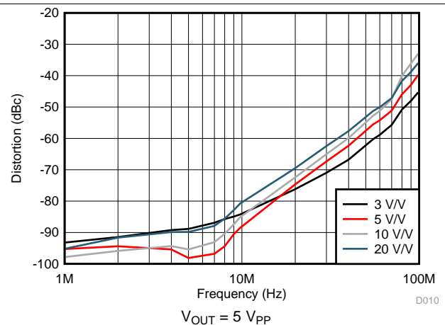
Figure 10. HD3 vs Gain
