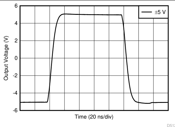
图 9-8. Pulse Response of the System With the Interstage Bessel Filter
