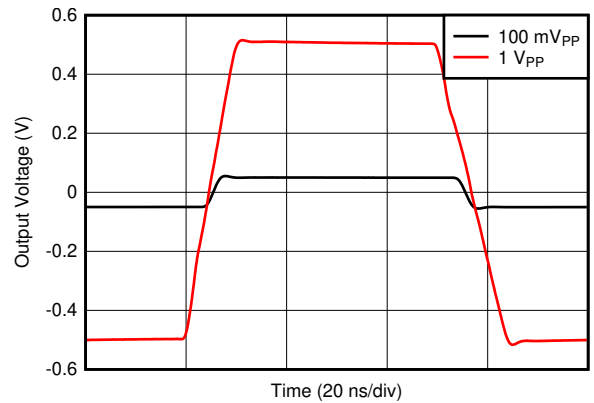
图 6-50. Step Response
