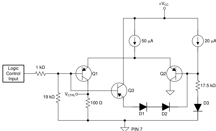
图 8-14. Logic Control Internal Schematic
