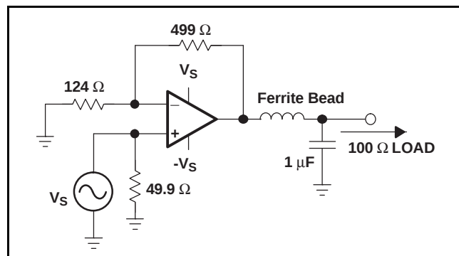
Figure 53. Ferrite Bead to Isolate Capacitive Load
