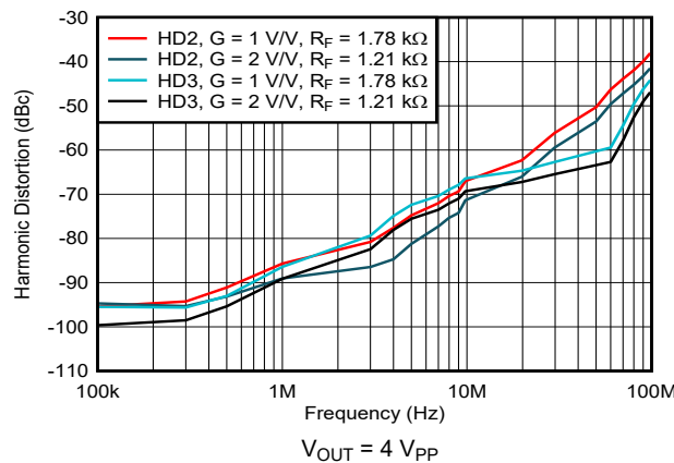
图 7-9. Harmonic Distortion vs Frequency
