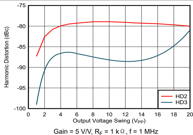
图 7-11. Harmonic Distortion vs Output Voltage Swing
