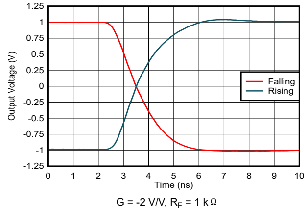
图 7-35. Settling Time
