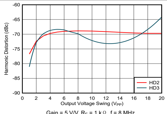
图 7-12. Harmonic Distortion vs Output Voltage Swing
