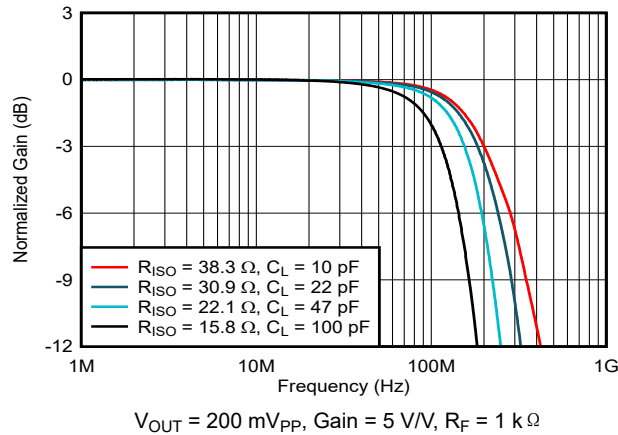
图 7-7. Capacitive Load Frequency Response
