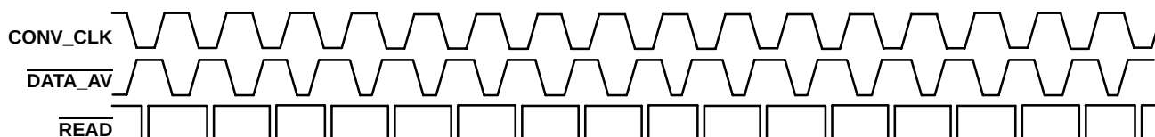
Figure 32. Trigger Level 1 Selected
