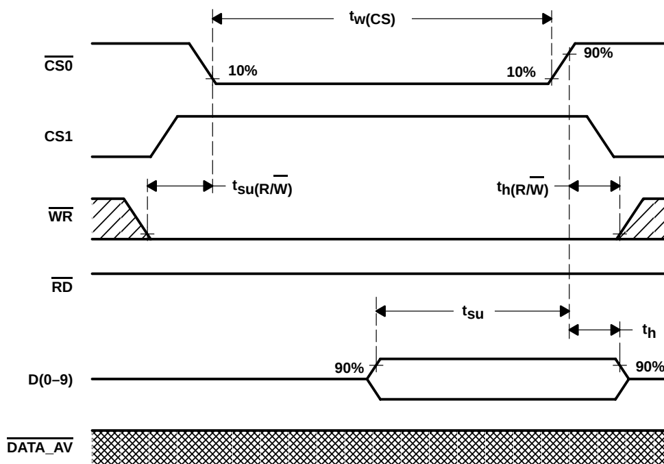
Figure 39. Write Timing Diagram Using \text{R}/\overline{\text{W}} ( \overline{\text{CS0}} -controlled)
