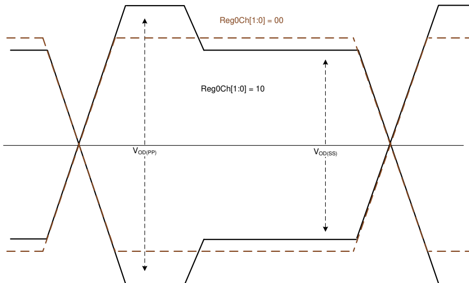
图 7-7. 6dB Pre-Emphasis in DP-Mode
