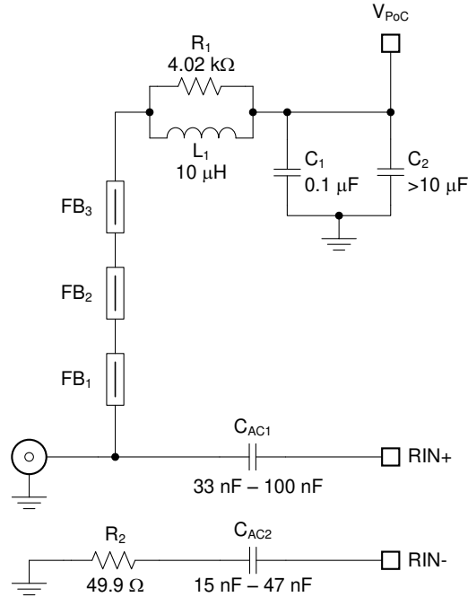
图 8-2. Example Recommended PoC Network for a "4G" V³Link
