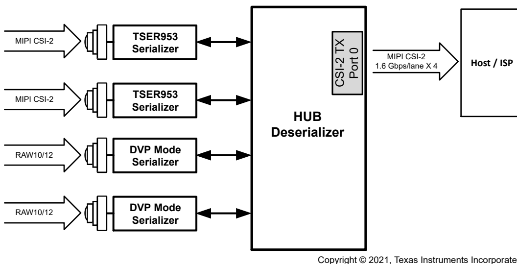
图 8-16. Two DVP Mode Serializers and Two TSER953 Sensor Data Onto CSI-2 Over 1 Port
