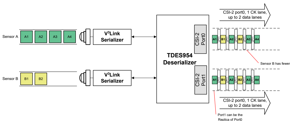
图 7-15. Two Sensor Data With Different Frame Size Replicated onto CSI-2 With Virtual Channels (VC-ID)
