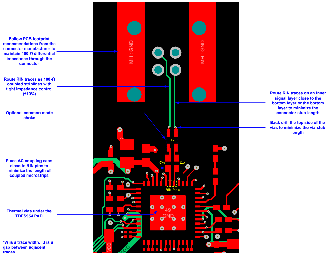
图 10-2. TDES954 PCB Layout Example: V³Link Differential Signal Traces
