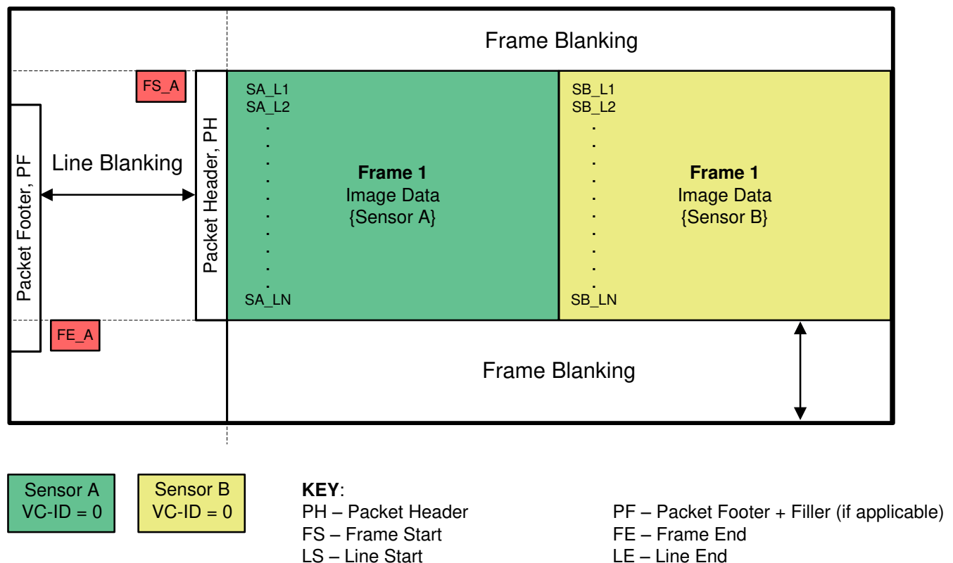
图 7-22. Line-Concatenated Format
