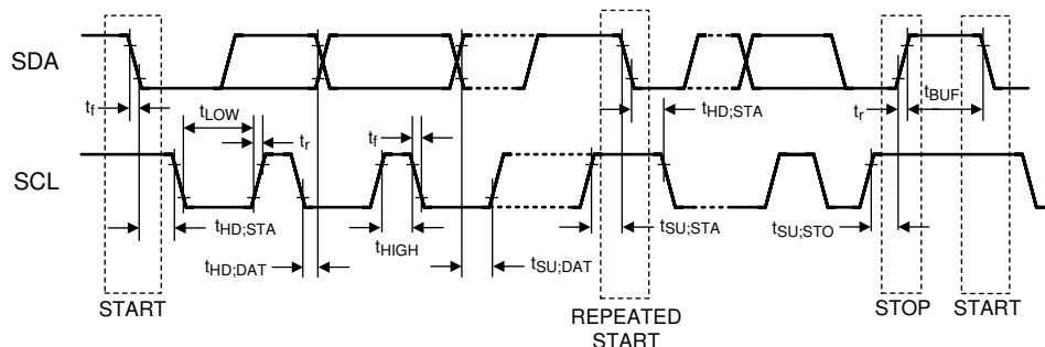
图 6-4. I²C Serial Control Bus Timing
