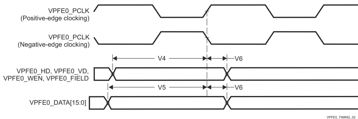
图 6-40. VPFE0 Timing Requirements
