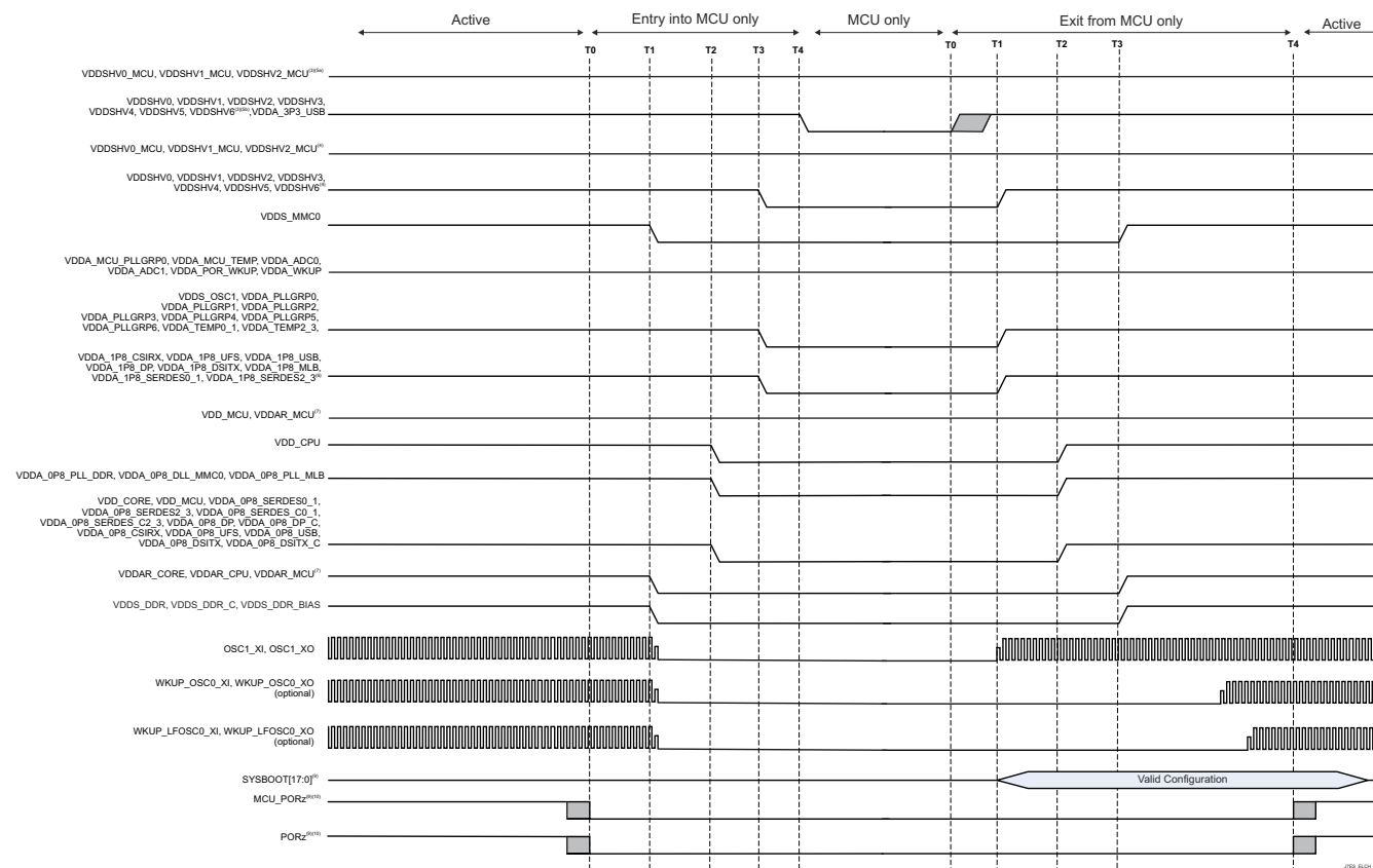
图 6-7. Entry and Exit of MCU Only Sequencing
