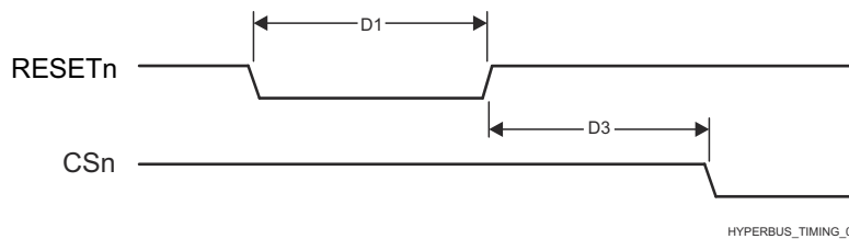
图 6-80. HyperBus Timing Diagrams - Reset
