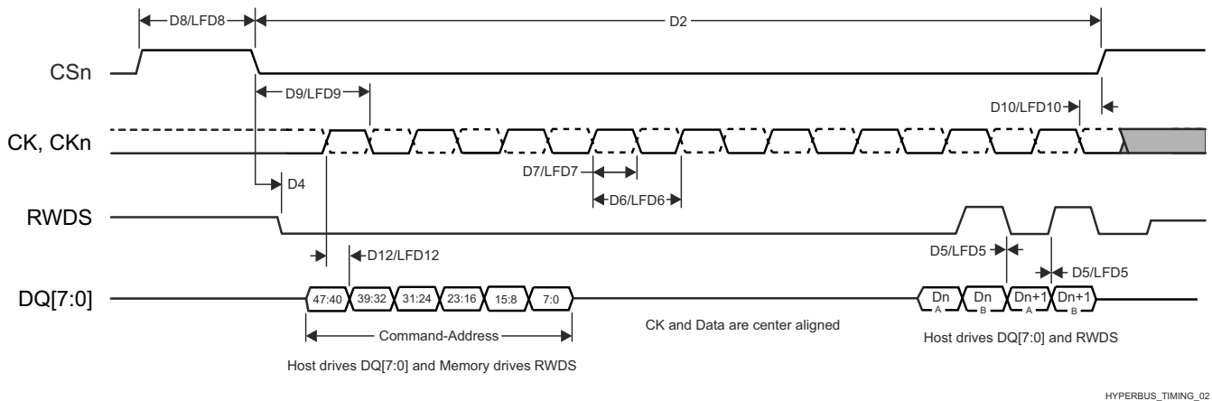
图 6-79. HyperBus Timing Diagrams - Receiver Mode
