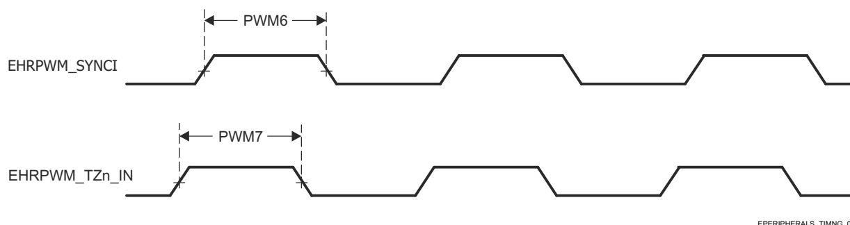
图 6-61. ePWM_SYNCI and ePWM_TZn_IN Output Timings
