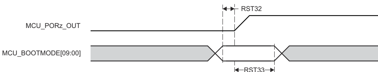
图 6-16. MCU_BOOTMODE Timing Requirements
