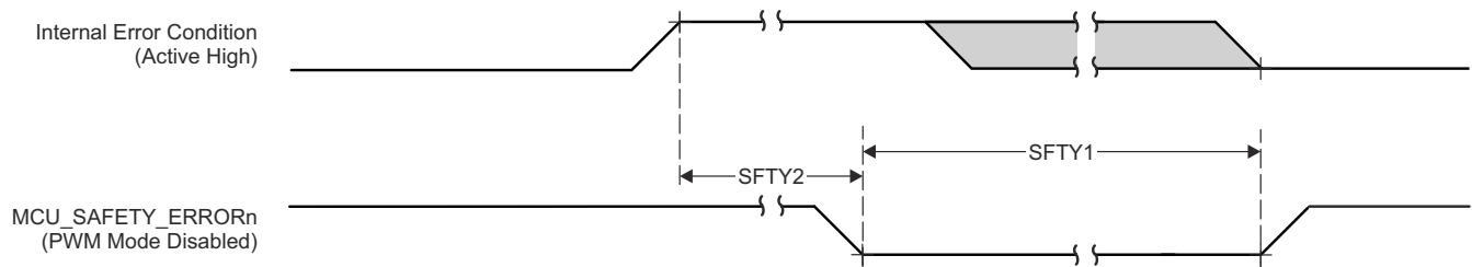
图 6-18. MCU_SAFETY_ERRORn Switching Characteristics
