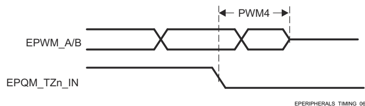
图 6-60. EPWM_A/B and ePWM_TZn_IN Hi - Z Input Timings
