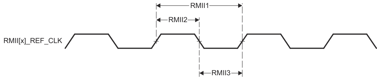
图 6-42. CPSW2G RMII[x]_REFCLK Timing Requirements - RMII Mode
