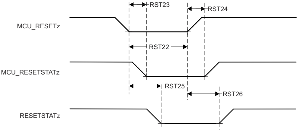
图 6-13. MCU_RESETz initiates; MCU_RESETSTATz, and RESETSTATz Timing Requirements and Switching Characteristics
