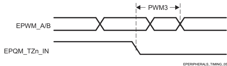
图 6-59. EPWM_A/B and ePWM_TZn_IN Forced High/Low Input Timings
