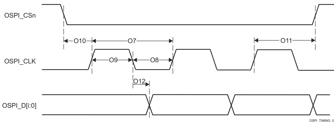
图 7-99. OSPI Switching Characteristics - SDR
