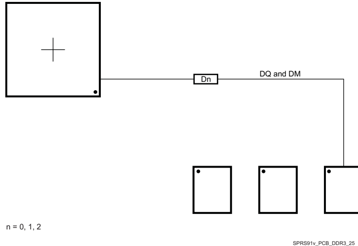
图 8-68. DQ/DM Routing With Any Number of Allowed DDR3 Devices
