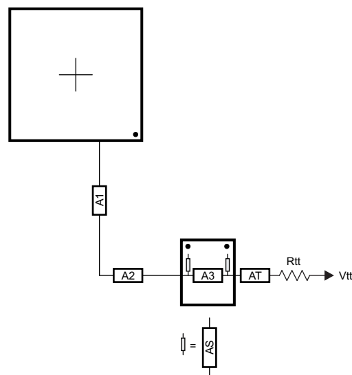
图 8-60. ADDR_CTRL Routing for Two Mirrored DDR3 Devices
