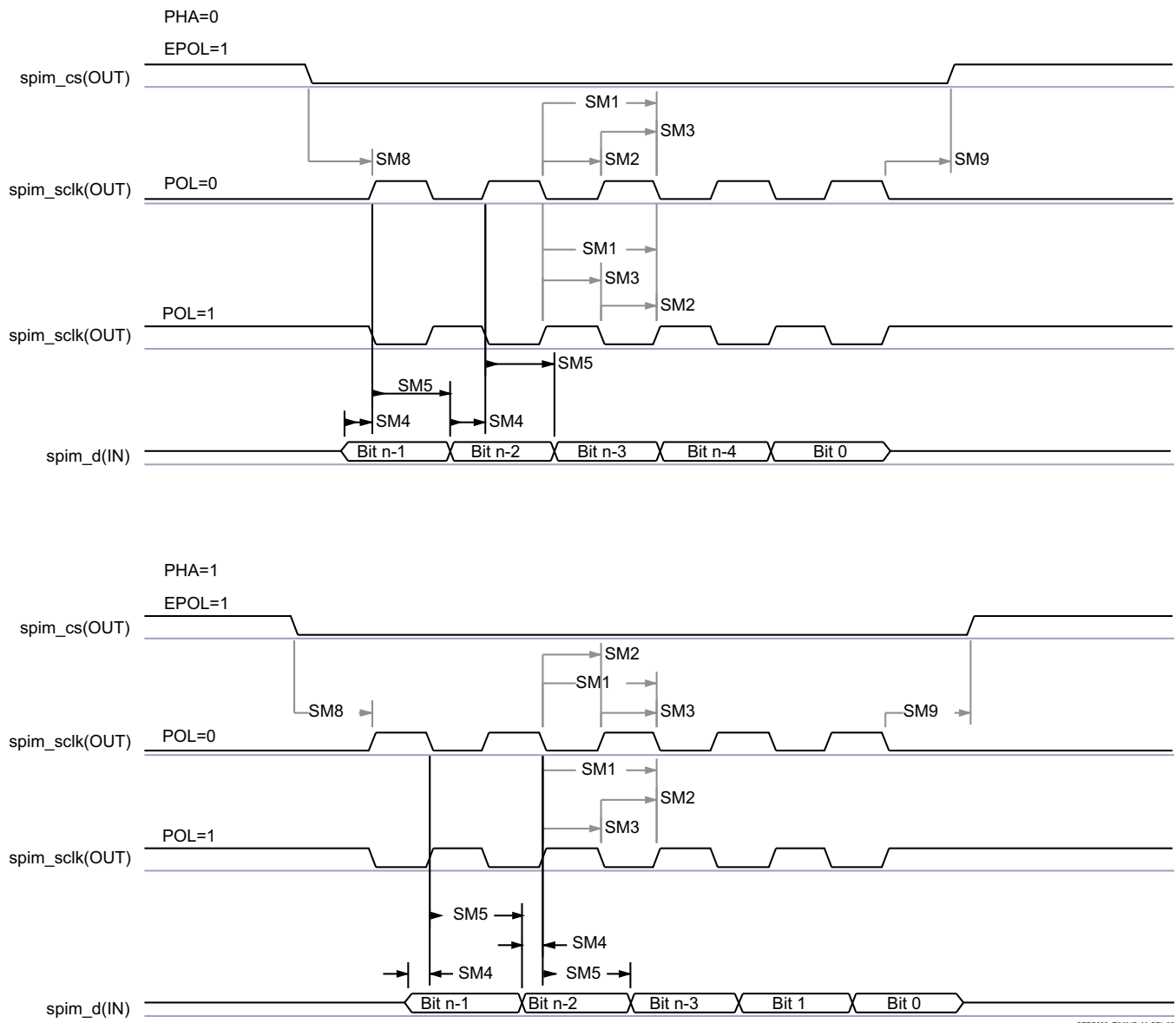
图 7-27. McSPI - Master Mode Receive
