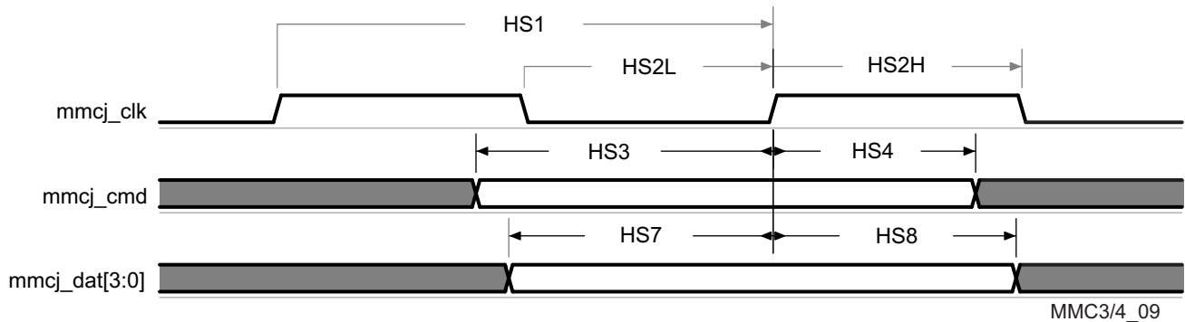
图 7-77. MMC/SD/SDIOj in - High Speed - Receiver Mode
