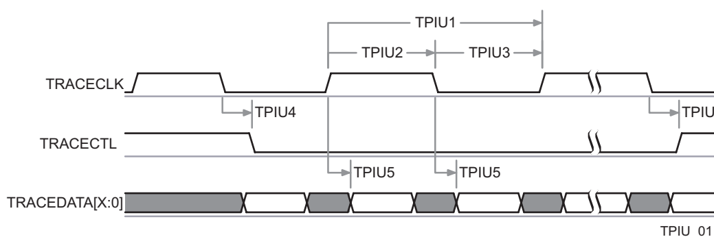
图 7-87. TPIU—PLL DDR Transmit Mode (1)
