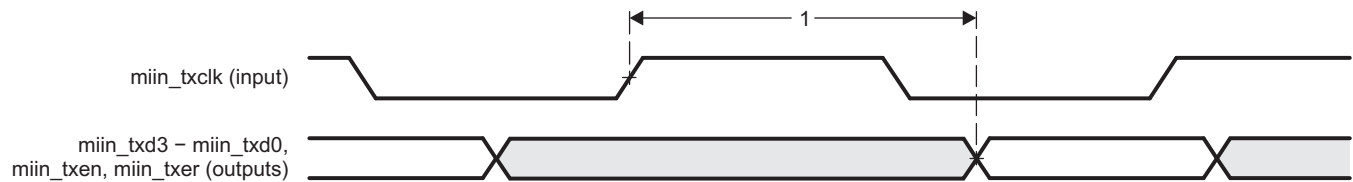
图 7-48. GMAC Transmit Interface Timing MII operation
