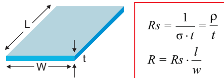
图 8-9. Depiction of Sheet Resistivity and Resistance
