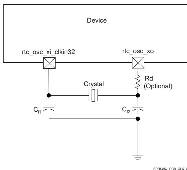
图 8-47. Grounding Scheme for Low-Frequency Clock
