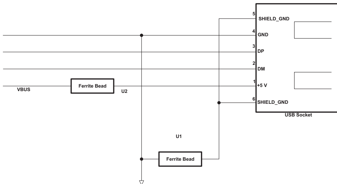
图 8-32. USB Connector
