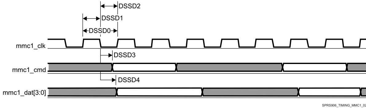
图 7-55. MMC/SD/SDIO in - Default Speed - Transmitter Mode
