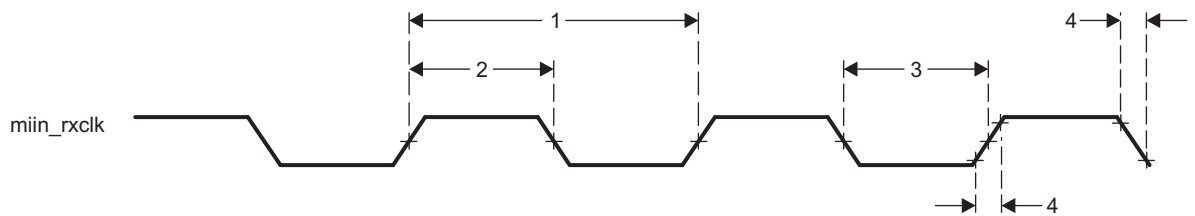
图 7-45. Clock Timing (GMAC Receive) - MII operation
