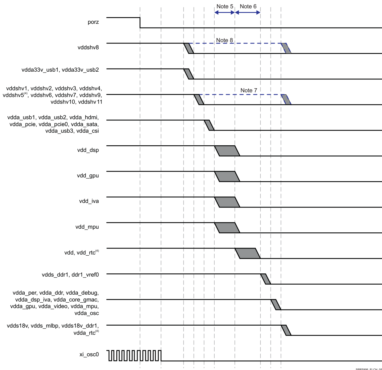
图 5-6. Power-Down Sequencing
