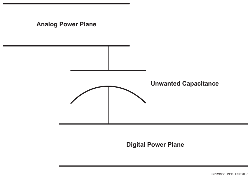
图 8-28. Do Not Overlap Planes
