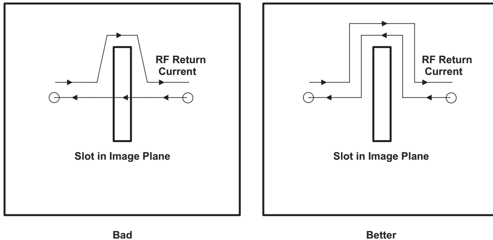
图 8-29. Do Not Violate Image Planes
