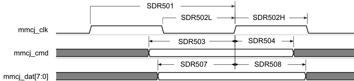
图 7-83. MMC/SD/SDIOj in - High Speed SDR50 - Receiver Mode
