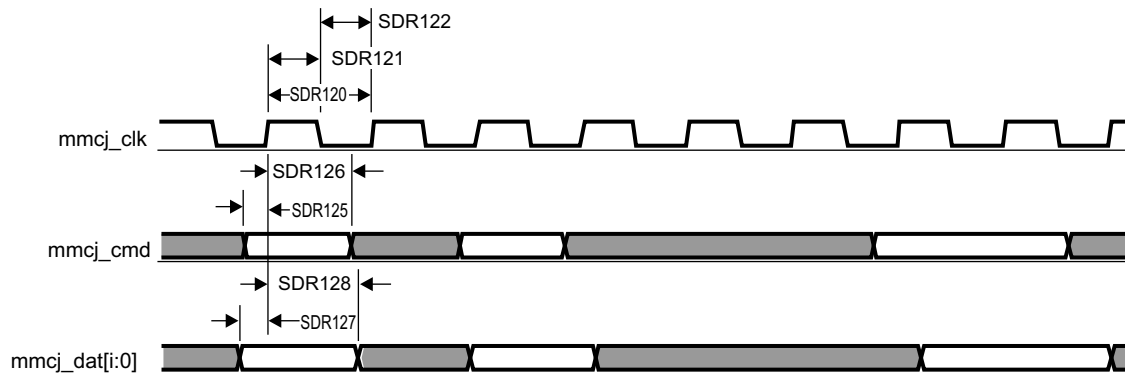
图 7-79. MMC/SD/SDIOj in - SDR12 - Receiver Mode
