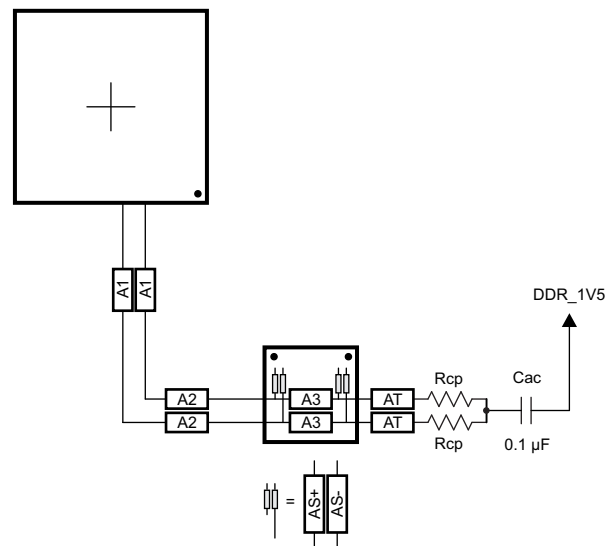
图 8-51. CK Routing for Two Mirrored DDR3 Devices
