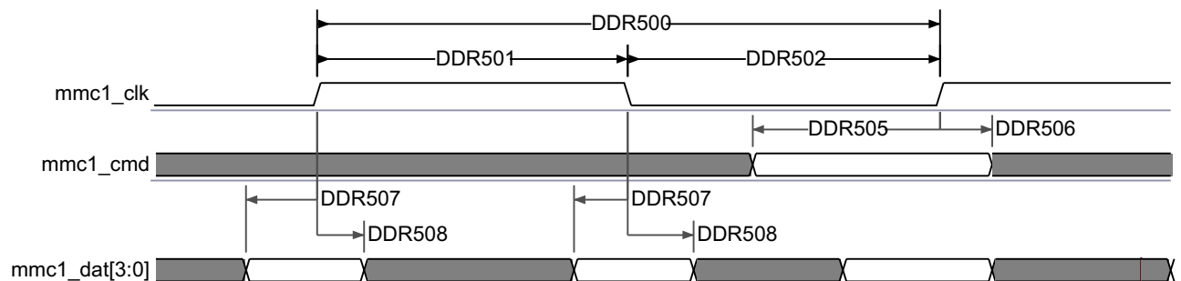
图 7-66. SDMMC - High Speed SD - DDR - Data/Command Receive
