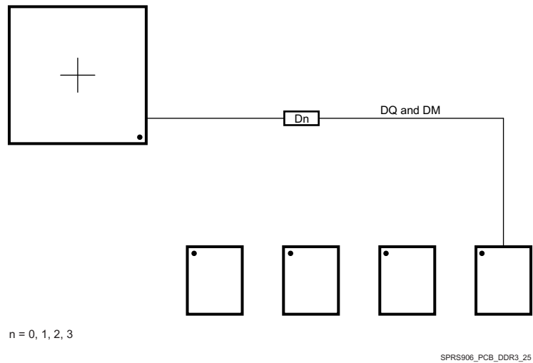
图 8-60. DQ/DM Routing With Any Number of Allowed DDR3 Devices
