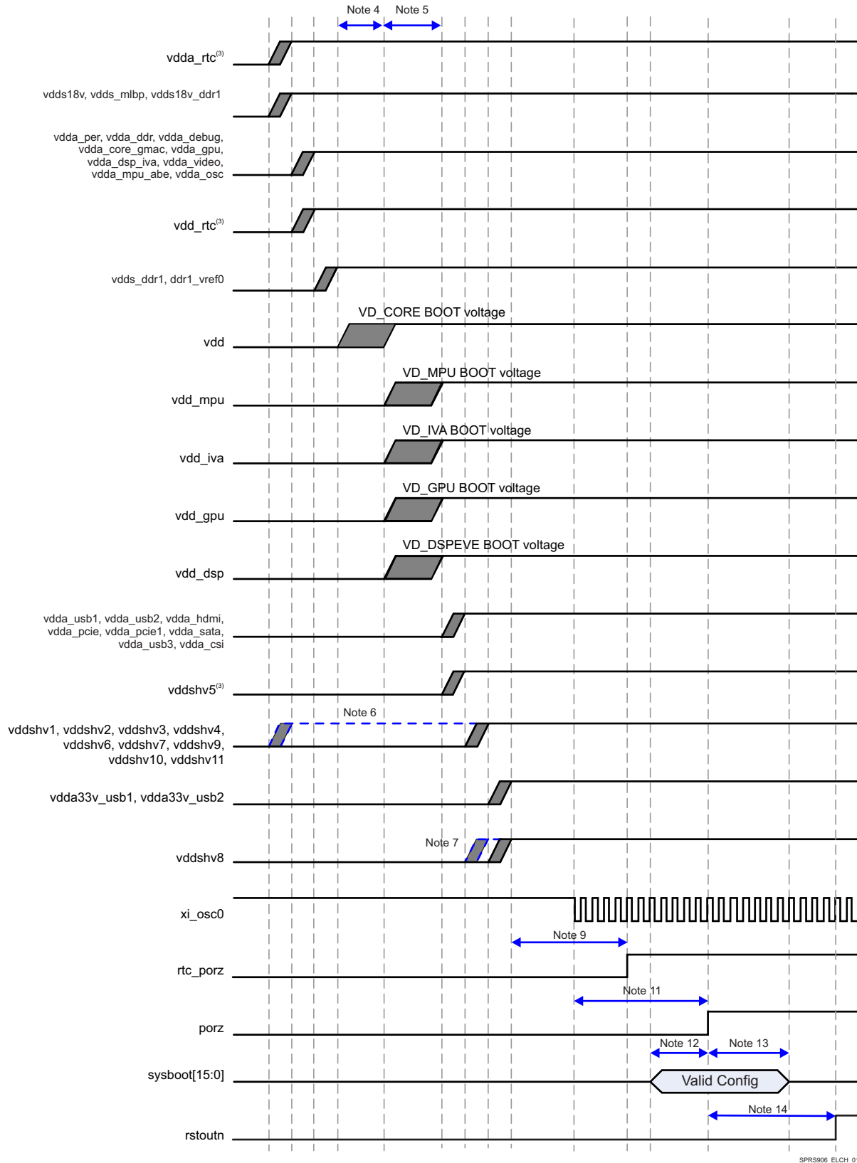
图 5-2. Power-Up Sequencing
