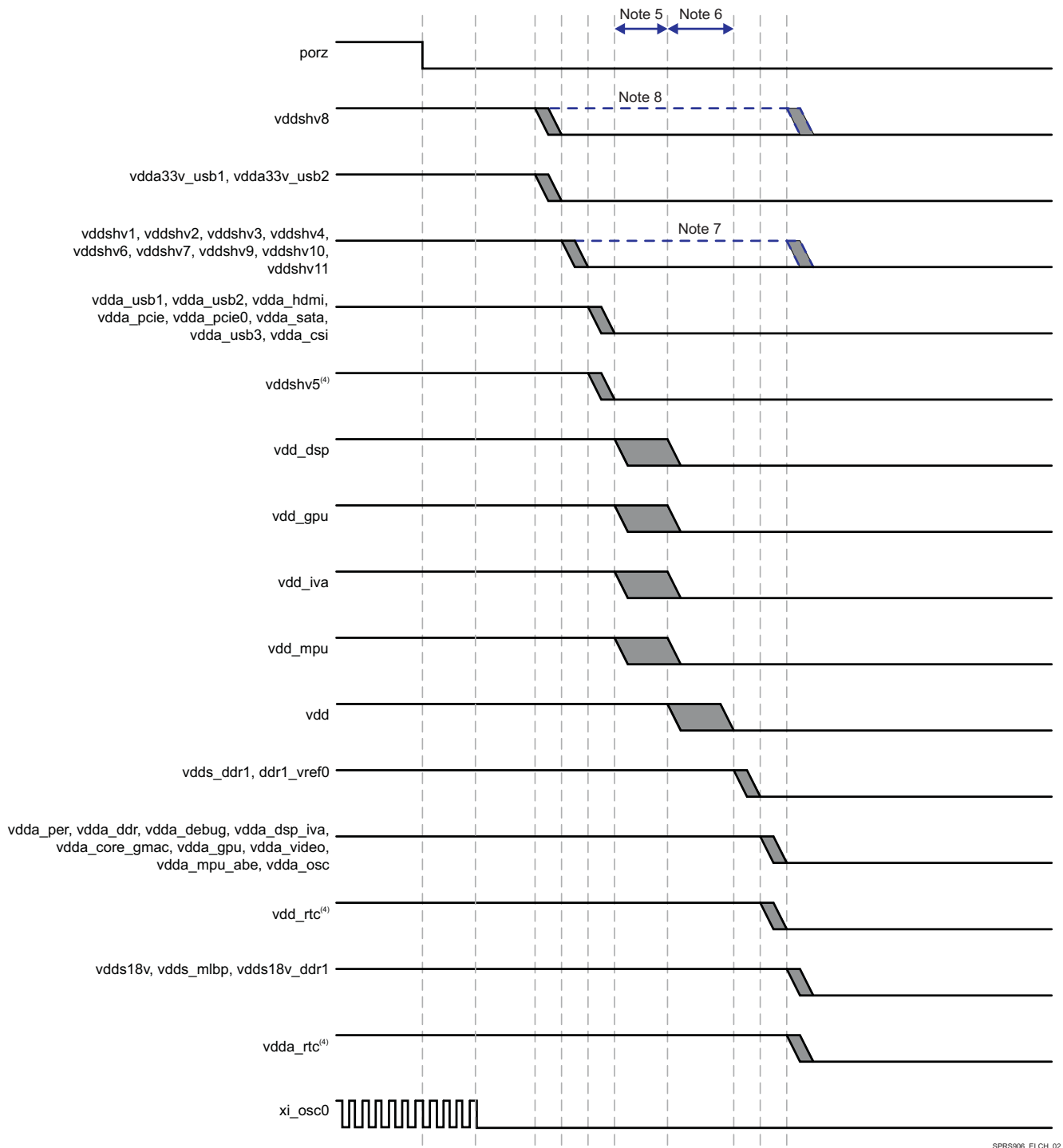
图 5-3. Power-Down Sequencing
