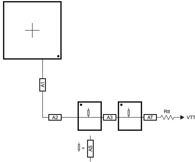
图 8-50. ADDR_CTRL Routing for Two Single-Side DDR3 Devices
