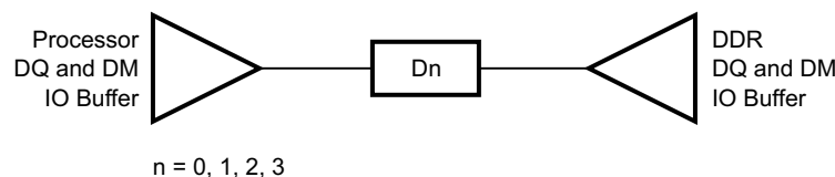
图 8-58. DQ/DM Topology
