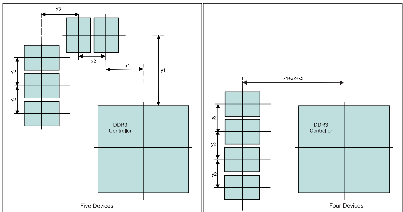
图 8-39. Placement Specifications
