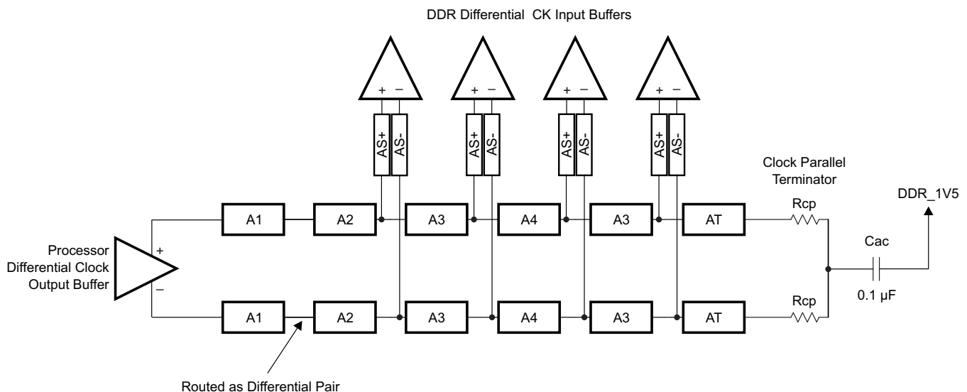
图 8-41. CK Topology for Four x8 DDR3 Devices
