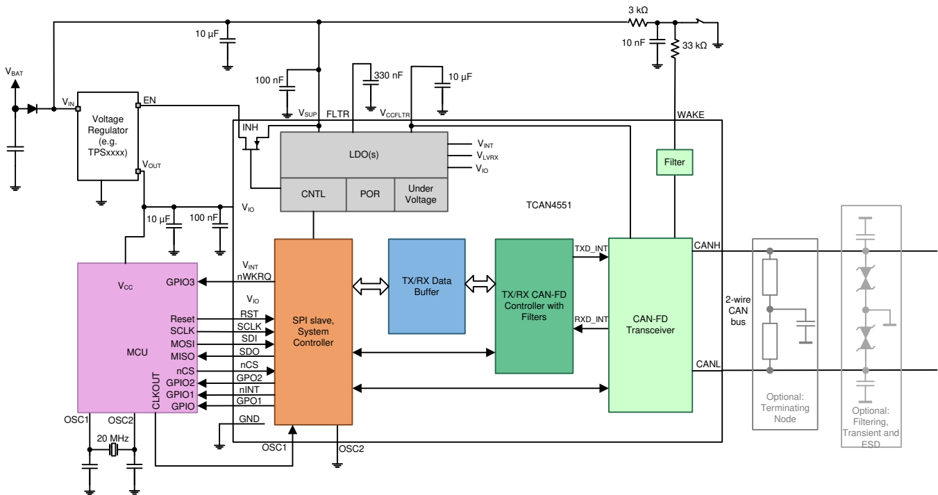
图 107. Typical CAN Applications for TCAN4551-Q1 for 3.3 V μC; Clock from MCU
