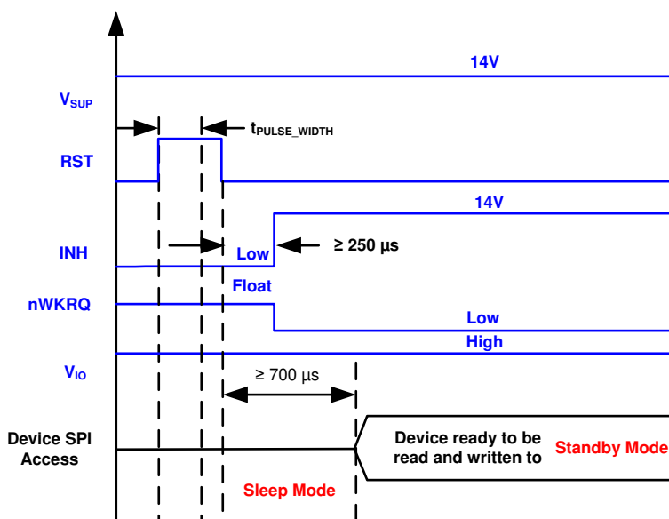
图 21. Timing for RST Pin in Sleep Mode
