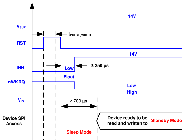
图 22. Timing for RST Pin in Sleep Mode
