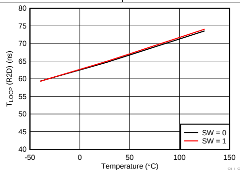
图 4. Dominant to Recessive T_{LOOP} over Temperature
