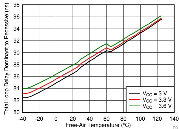
图 5-17. Total Loop Delay Dominant to Recessive t_{PROP(LOOP2)} vs Free-Air Temperature
