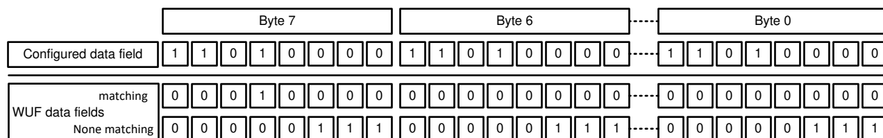
图 8-20. Data Field Validation for WUF Example
