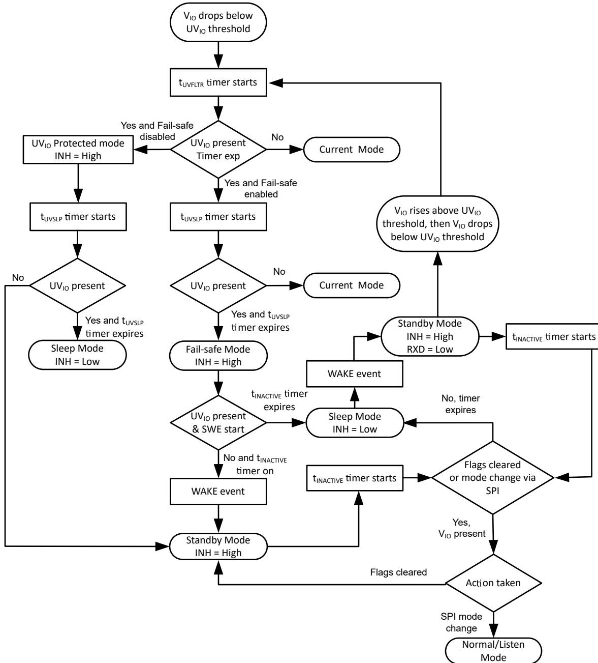
图 8-25. UV IO State Diagram
