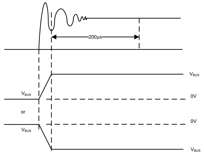
图 7-8. Driver Short-Circuit Current Test and Measurement
