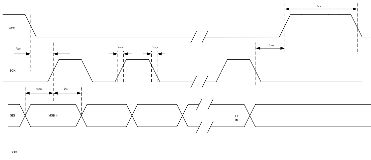
图 7-10. SPI AC Characteristic Write
