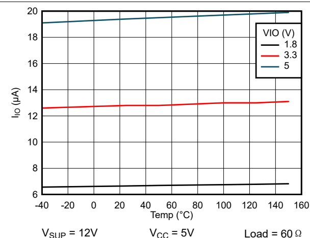
图 6-5. Normal Mode Dominant: I_{IO} vs Temperature
