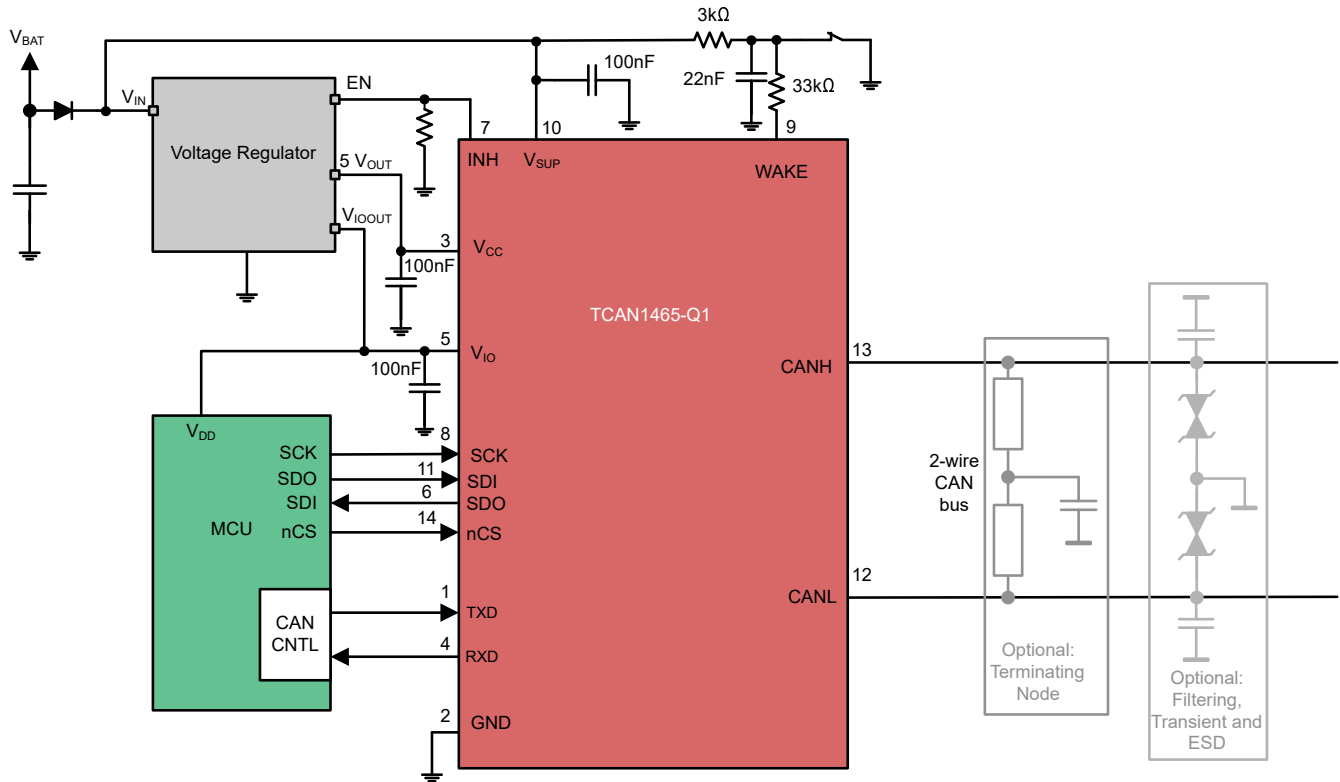
图 9-5. Typical CAN Application for TCAN1465-Q1
