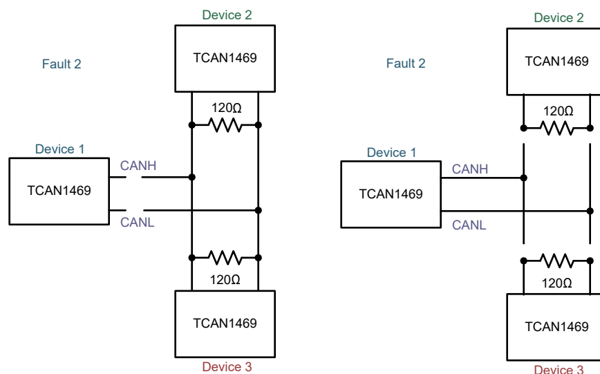
图 8-35. Open Fault 2 Examples
