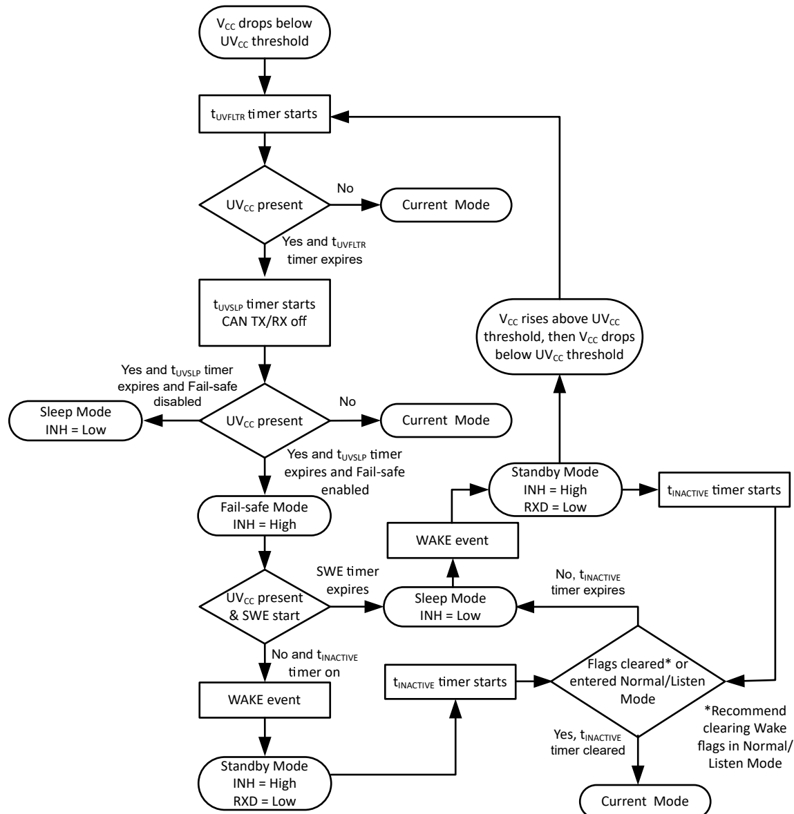
图 8-24. UV CC State Diagram
