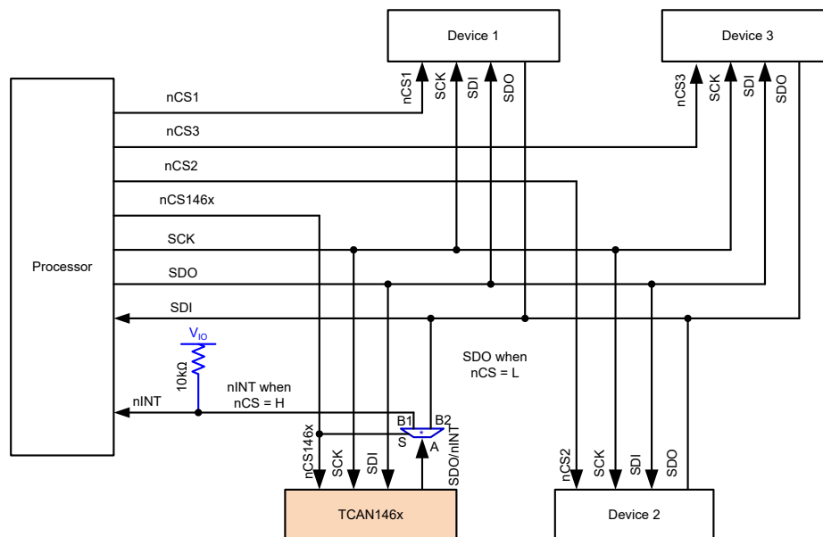
图 8-6. Example System Using nINT Feature
