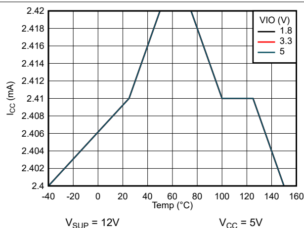
图 6-1. Normal Mode Recessive I_{CC} vs Temperature
