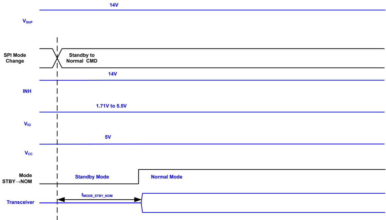
图 7-16. Standby to Normal Timing
