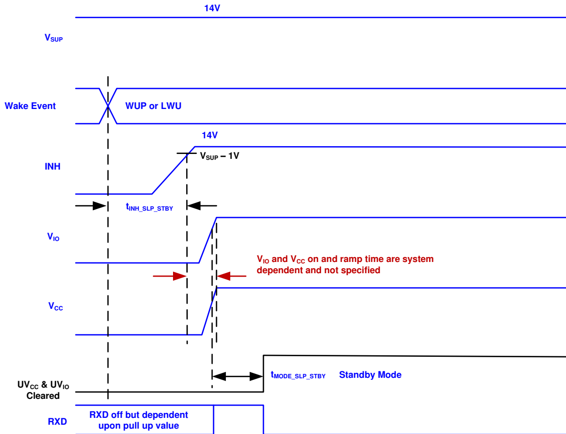
图 7-13. Sleep to Standby Timing
