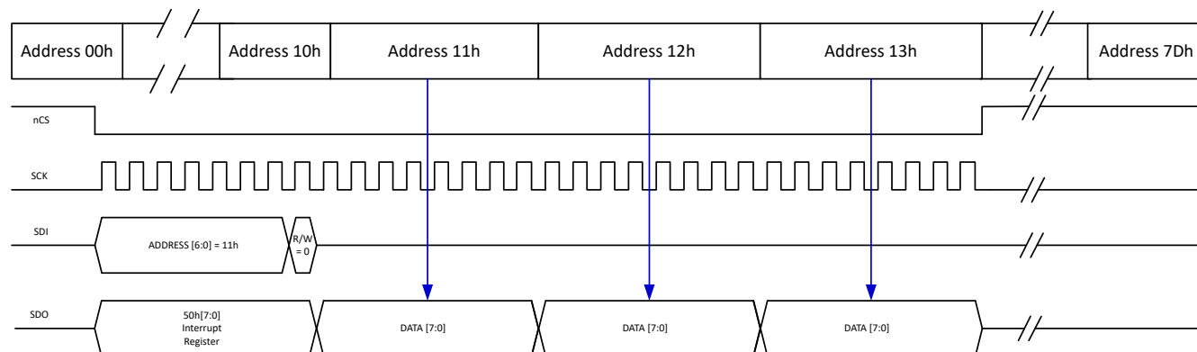
图 8-44. 32-bit SPI Burst Read
