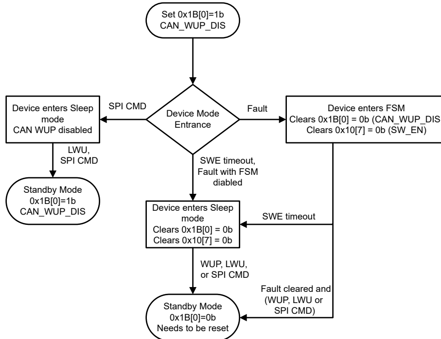
图 8-8. CAN Bus Wake Up Pattern Disable
