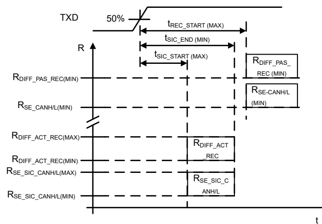
图 7-17. Resistance Value During Active Recessive Phase for Signal Improvement Capability
