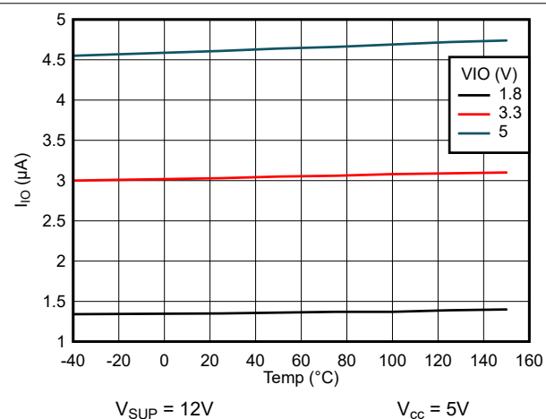
图 6-4. Normal Mode Recessive I_{IO} vs Temperature
