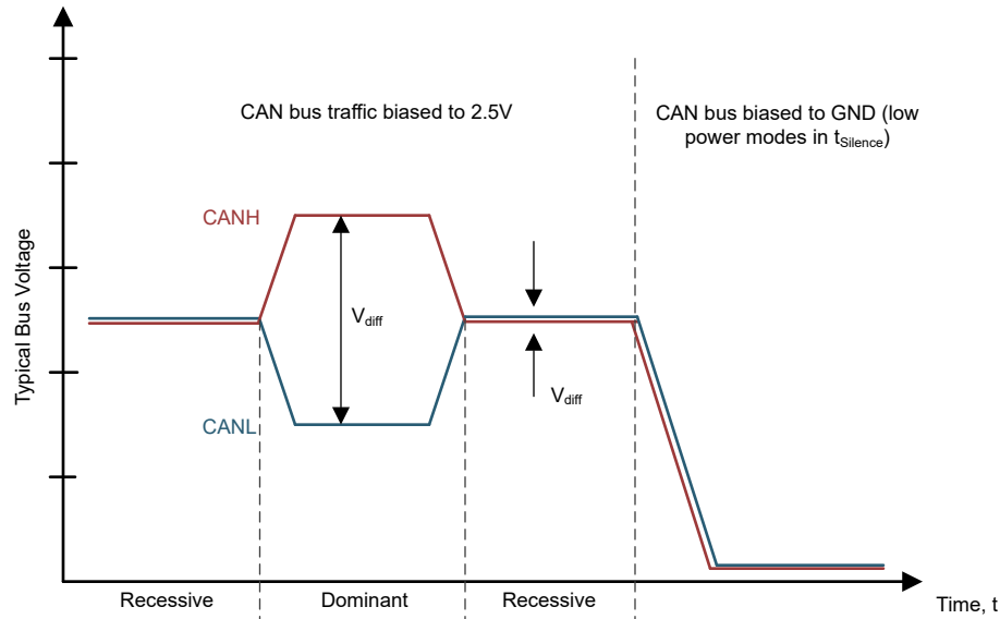
图 7-1. Bus States (Physical Bit Representation)
