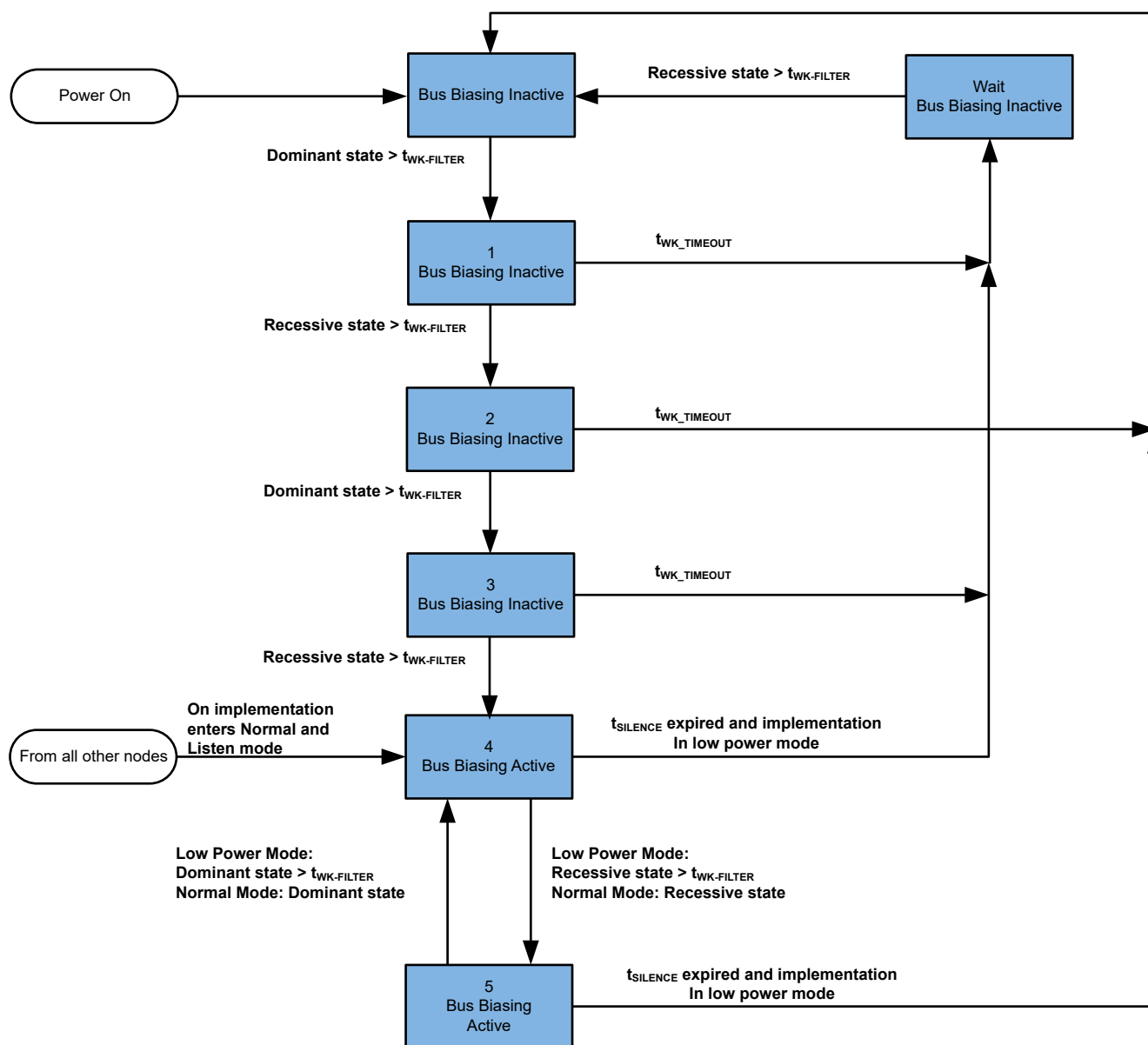
图 9-3. Automatic bus biasing state diagram
