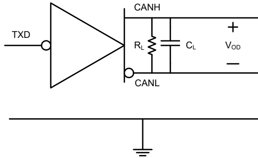
图 7-7. TXD Dominant Time Out Test Circuit and Measurement
