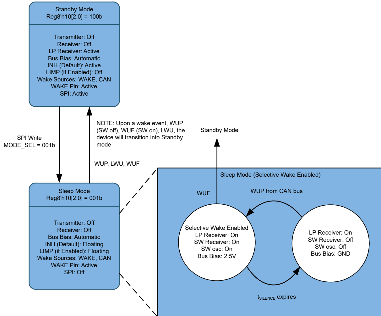
图 8-12. Selective Wake Enabled Sleep Mode
