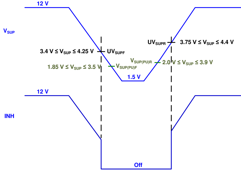
图 9-7. INH Behavior During Brownout
