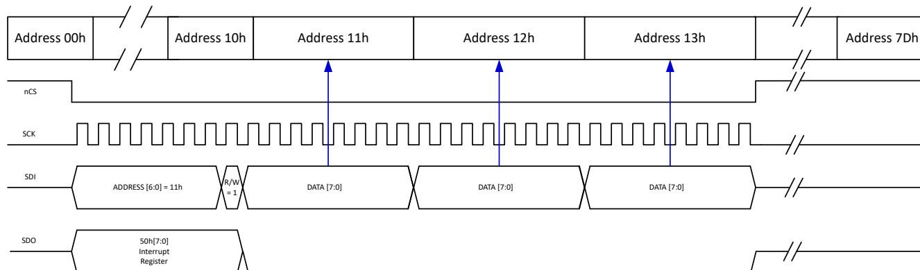
图 8-42. 32-bit SPI Burst Write
