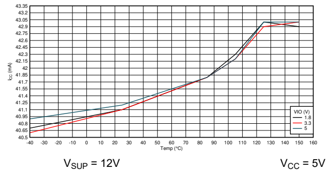
图 9-9. Normal Mode: I_{CC} vs Temperature Dominant
