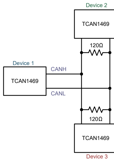
图 8-34. Three-Node Example
