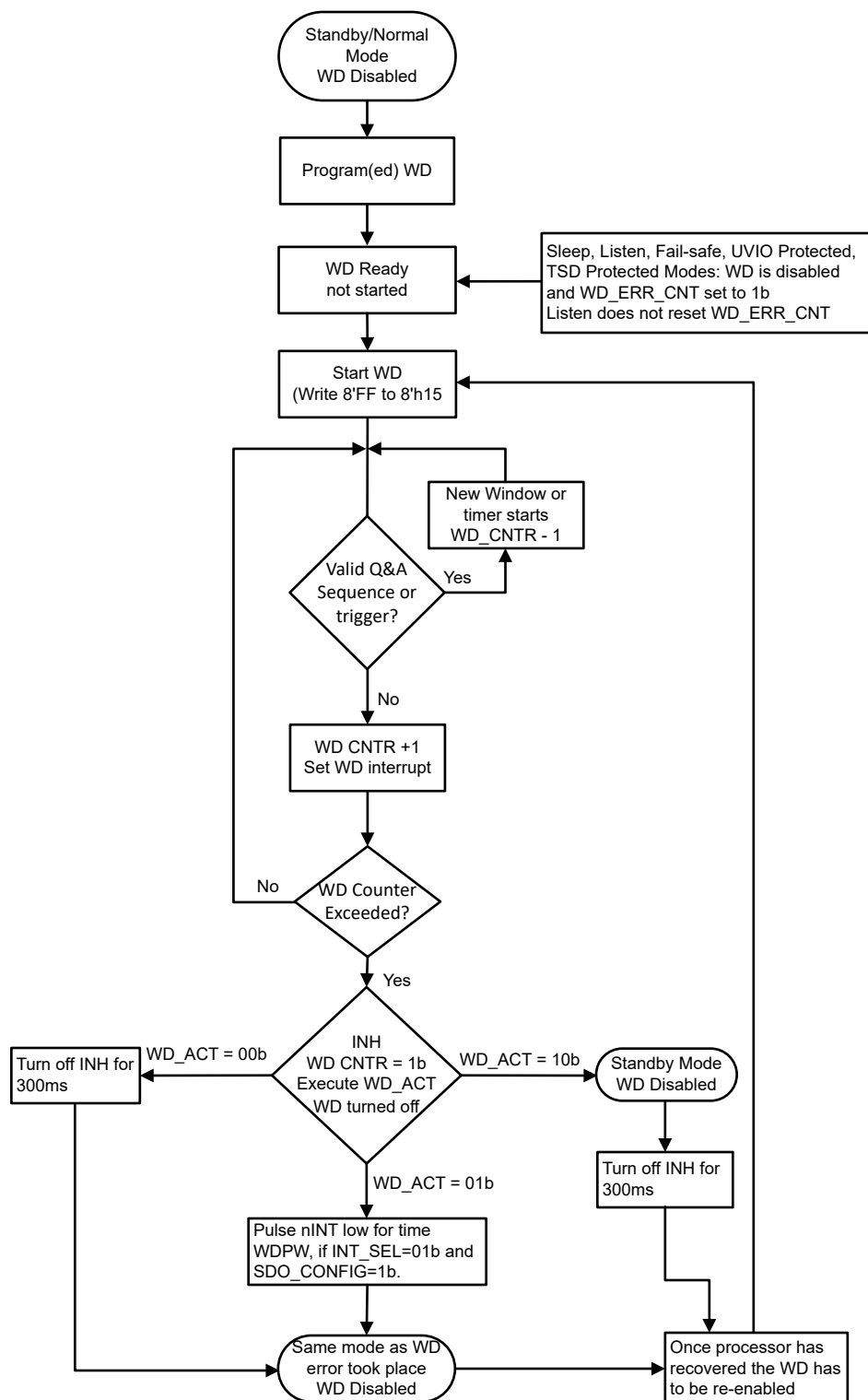
图 8-26. Watchdog Flow Chart INH Pin
