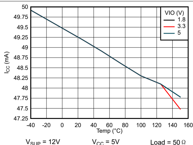
图 6-3. Normal Mode Dominant I_{CC} vs Temperature
