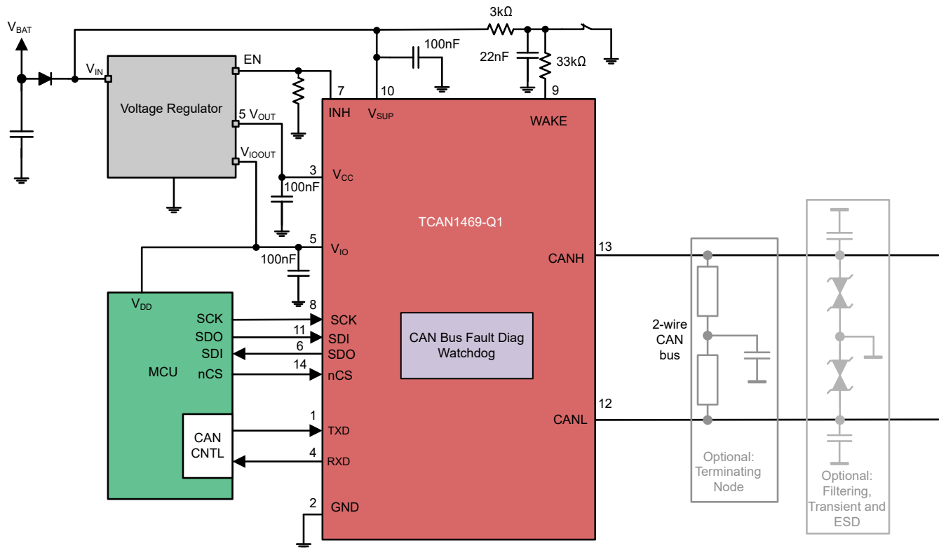
图 9-6. Typical CAN Application for TCAN1469-Q1
