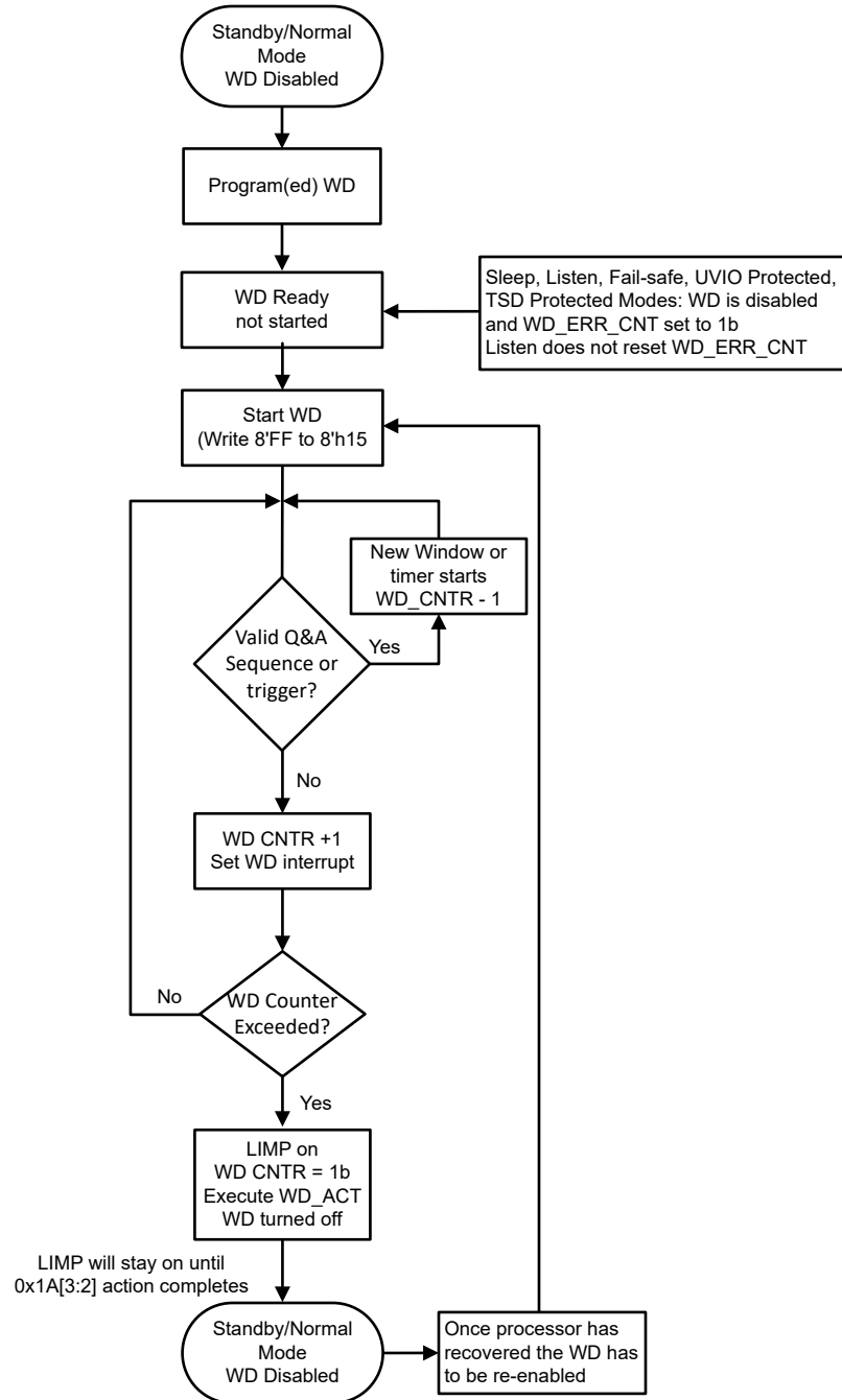
图 8-27. Watchdog Flow Chart LIMP Pin
