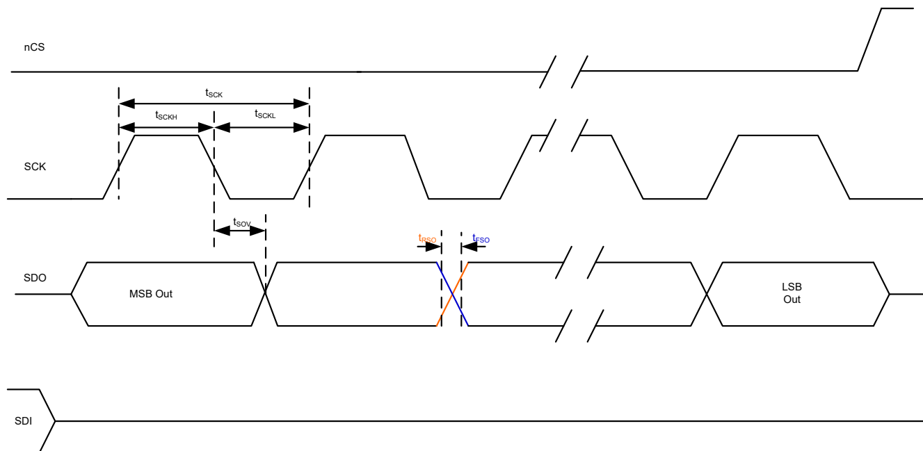
图 7-11. SPI AC Characteristic Read
