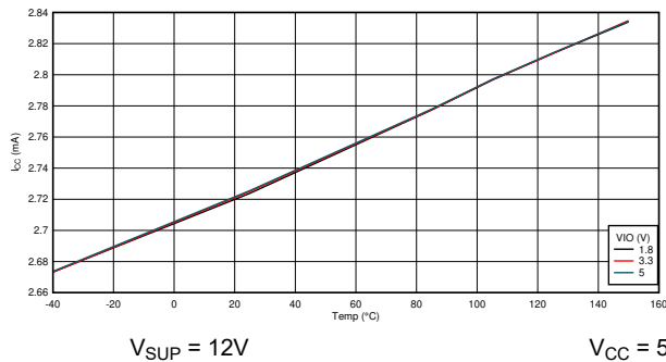
图 9-8. Normal Mode: I_{CC} vs Temperature Recessive
