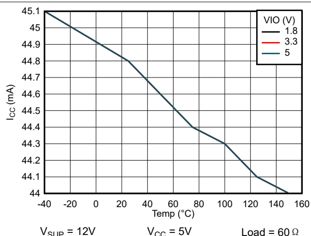
图 6-2. Normal Mode Dominant I_{CC} vs Temperature
