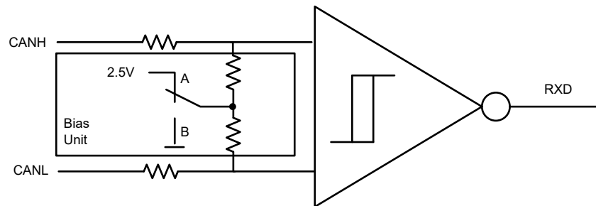
图 7-2. Simplified Recessive Common Mode Bias Unit and Receiver
