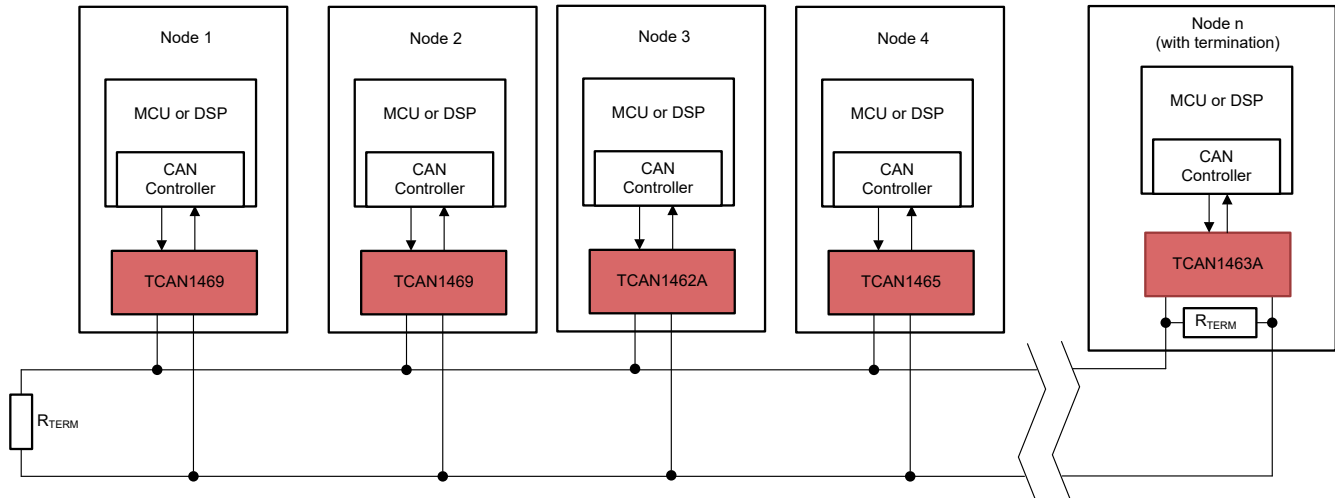
图 9-1. Typical CAN Bus
