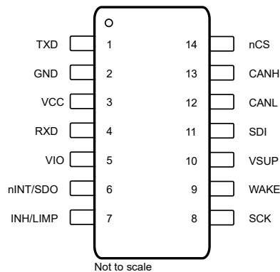
图 5-3. DYY Package, 14 Pin (SOT-23), Top View
