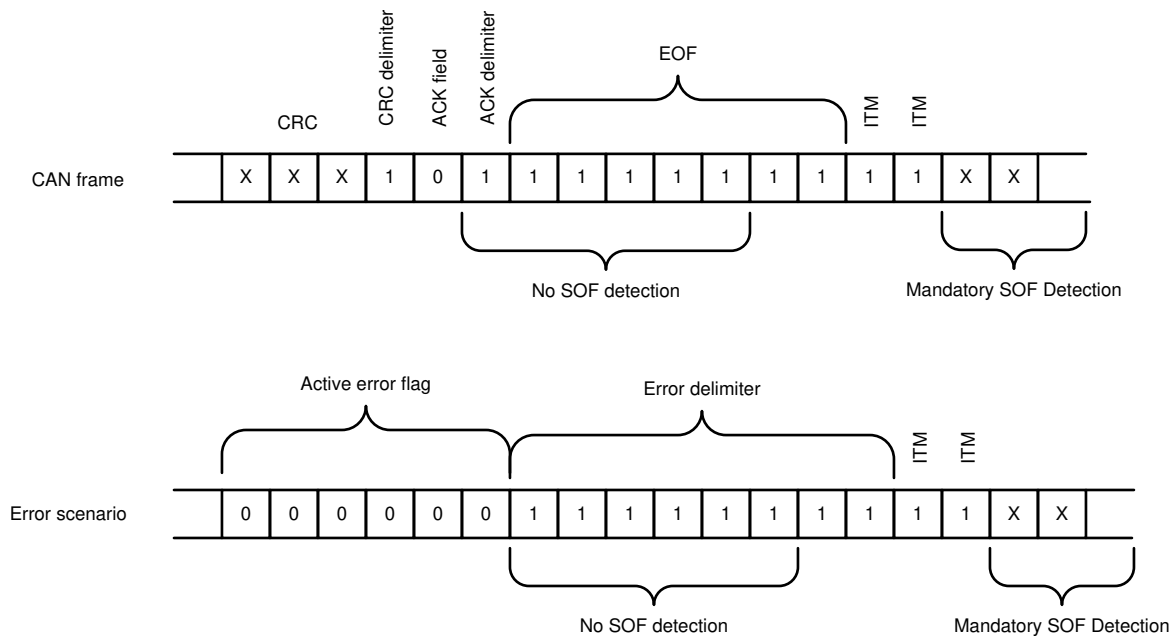
图 8-22. Mandatory SOF Detection after Classic CAN Frames and Error Scenarios
