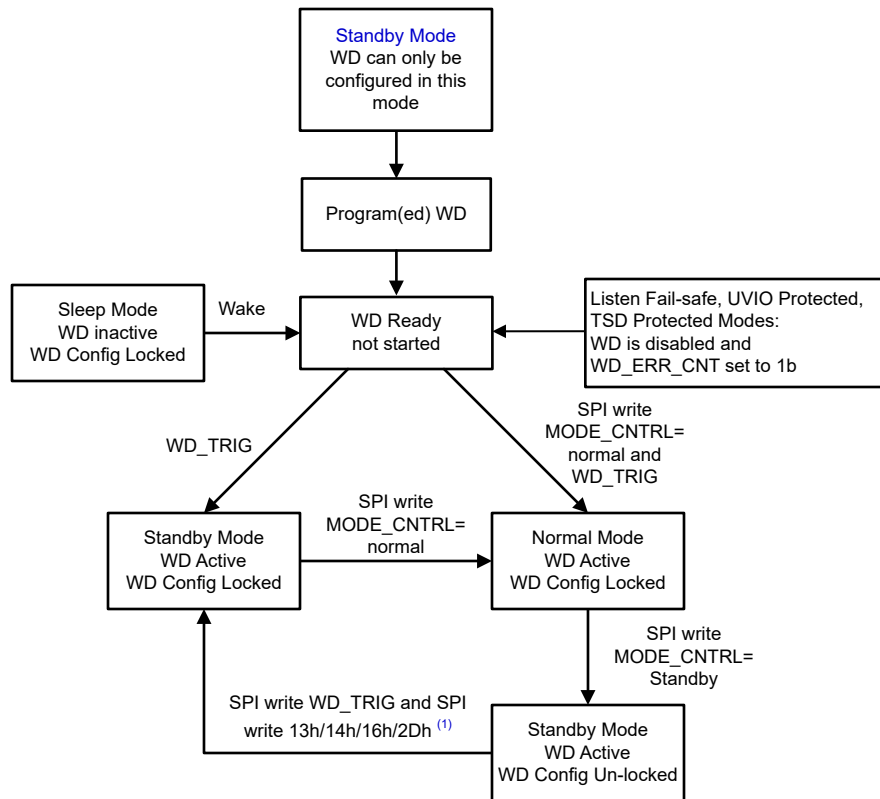
图 8-28. Watchdog Lock and Unlock Flow Chart
