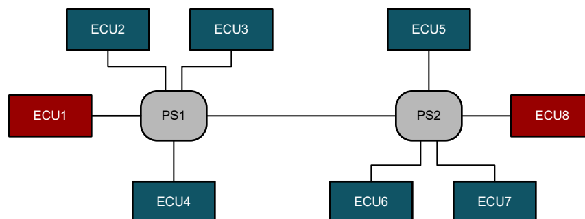
图 8-9. CAN FD Signal Improvement Topology
