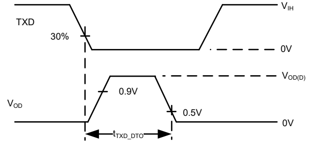
图 7-7. TXD Dominant Time Out Test Circuit and Measurement
