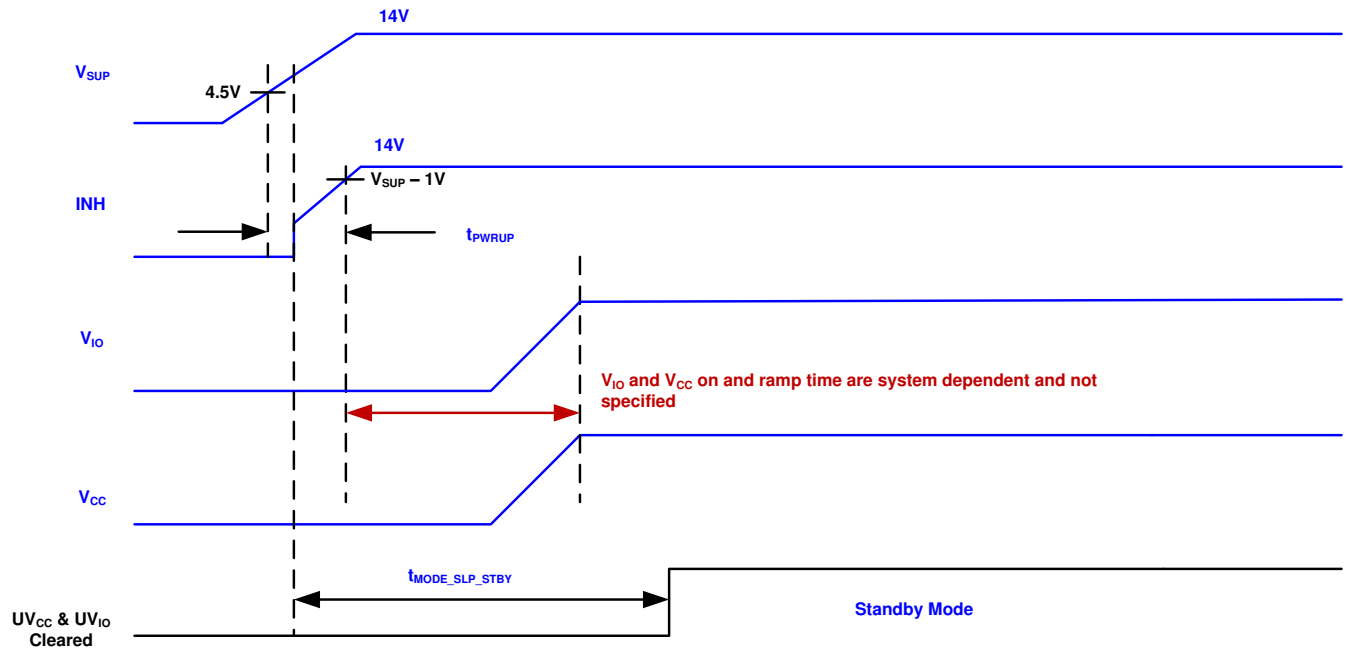
图 7-12. Power Up Timing
