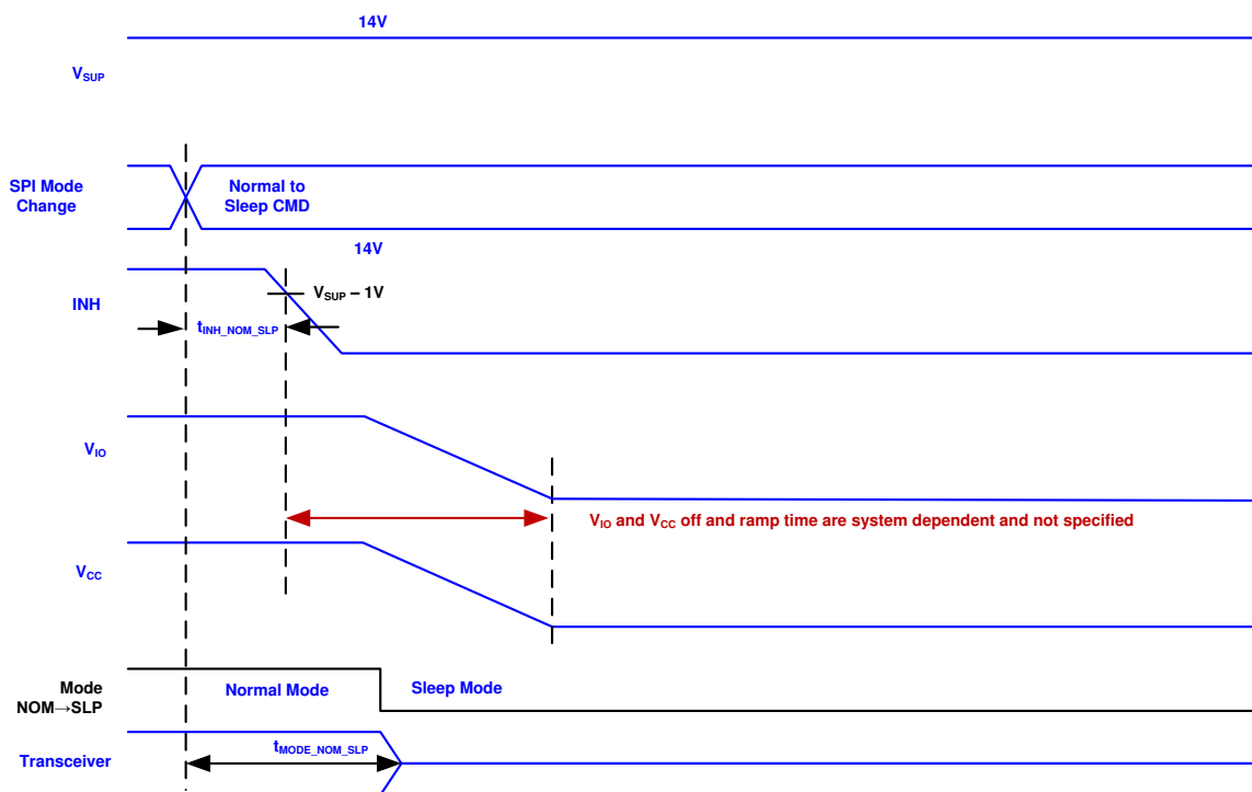
图 7-14. Normal to Sleep Timing
