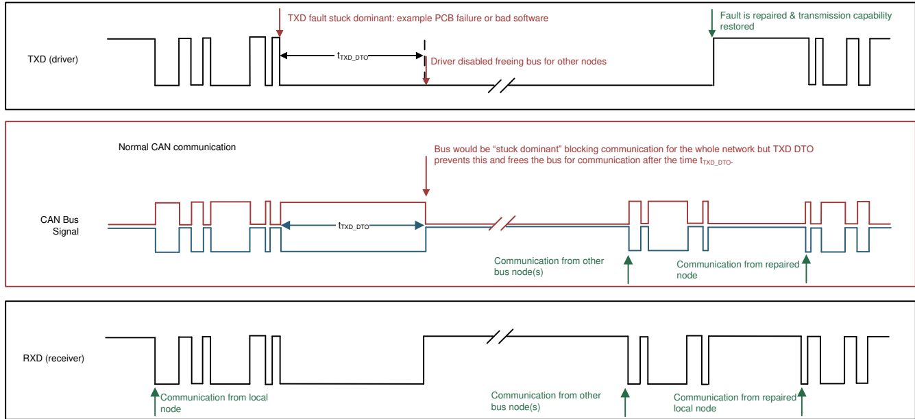
图 8-14. Example timing diagram with TXD DTO
