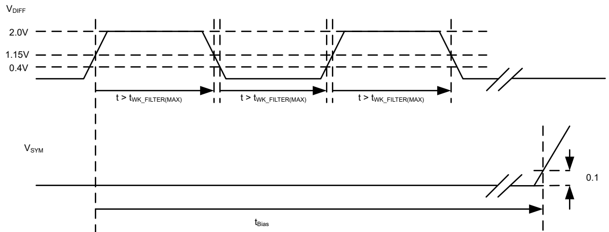
图 7-9. Test Signal Definition for Bias Reaction Time Measurement
