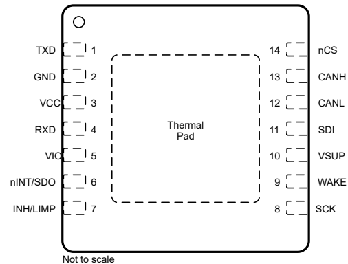
图 5-2. DMT Package, 14 Pin (VSON), Top View
