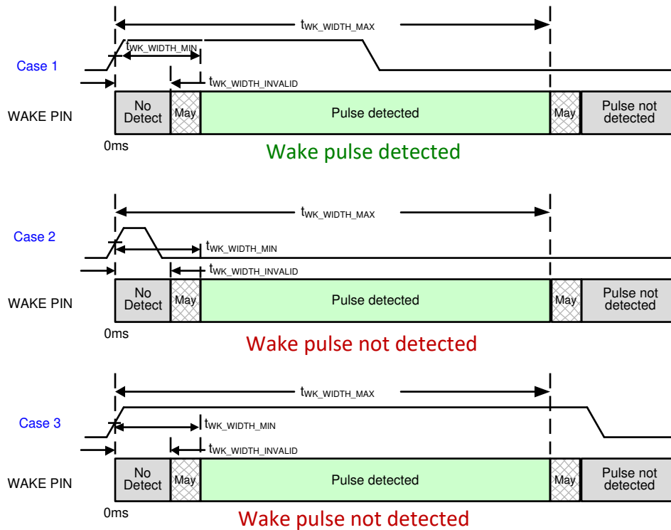
图 8-17. WAKE Pin Pulse Behavior
