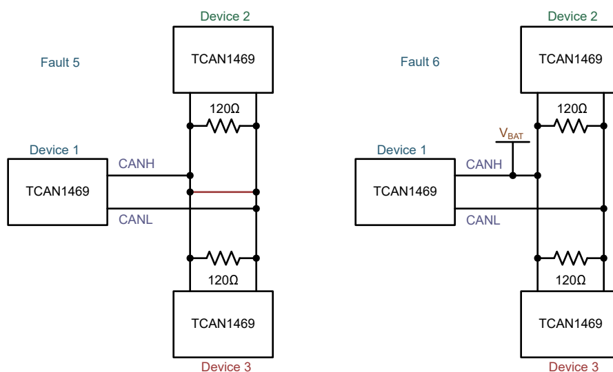
图 8-37. Fault 5 and 6 Examples
