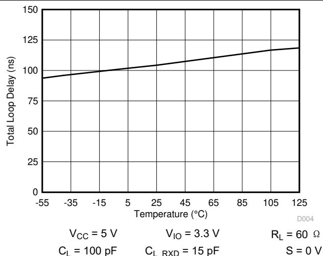
图 6-4. Total Loop Delay over Temperature
