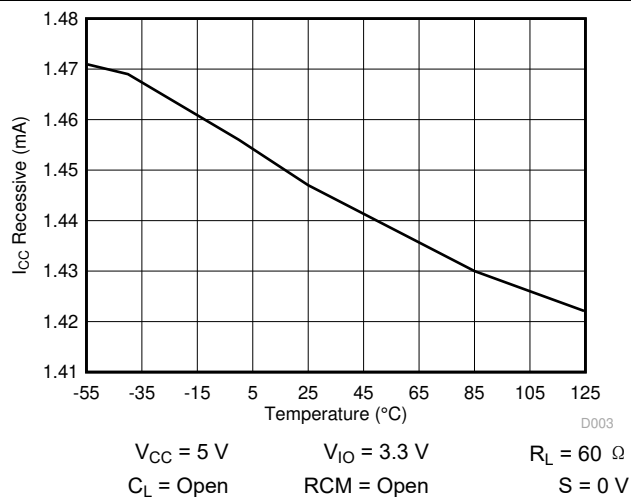
图 6-3. I_{CC} Recessive over Temperature
