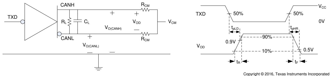
图 7-1. Driver Test Circuit and Measurement
