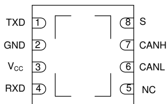
图 5-2. DRB Package for Base, (H), (G), and (HG) Devices 8 PIN (VSON) Top View
