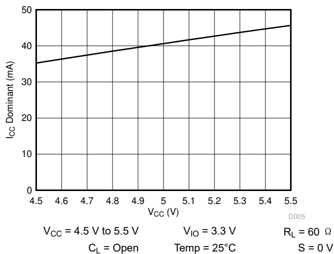
图 9-5. I CC Dominant Current over V CC Supply Voltage
