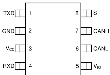
图 5-3. D Package for (V), (GV), (HV) and (HGV) Devices 8 PIN (SOIC) Top View
