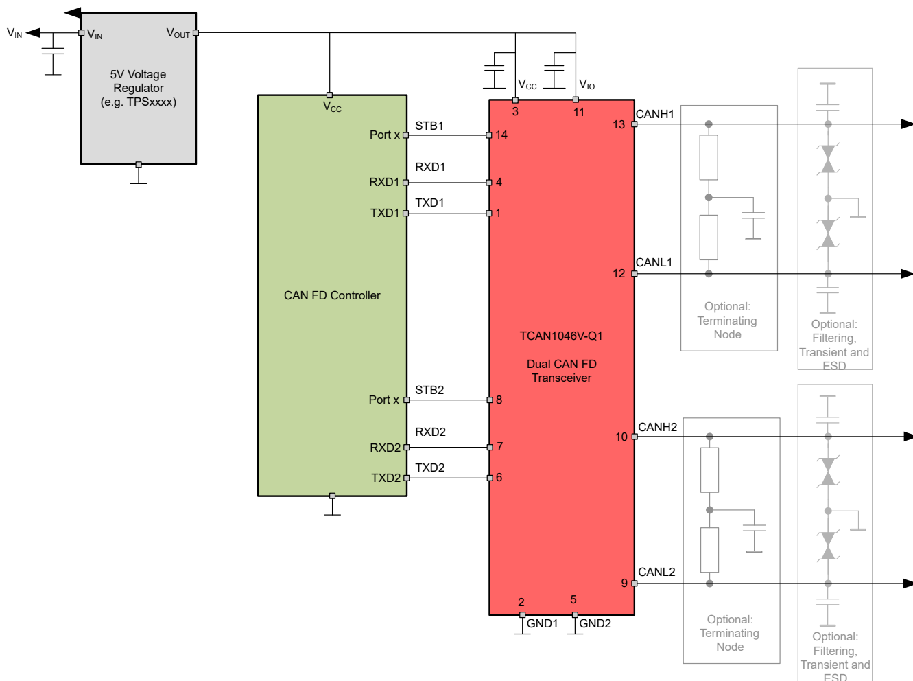
图 9-1. Transceiver Application Using 5 V I/O Connections
