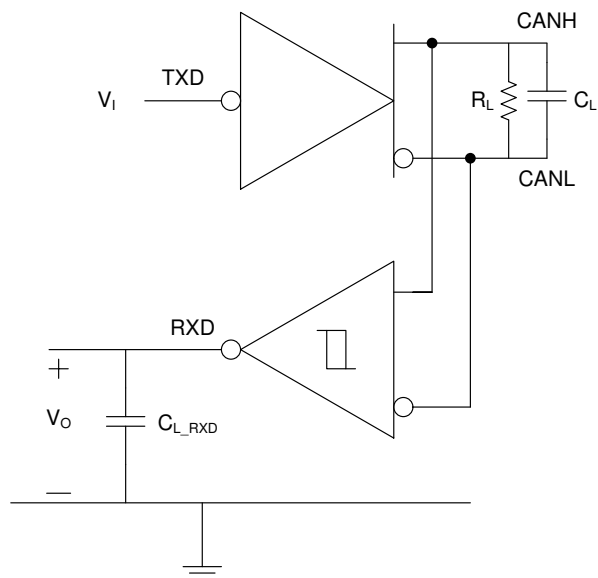
图 7-6. t_{\text{PROP(LOOP)}} Test Circuit and Measurement
