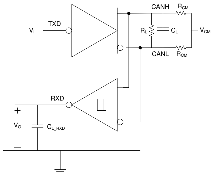
图 7-6. t_{\text{PROP(LOOP)}} Test Circuit and Measurement
