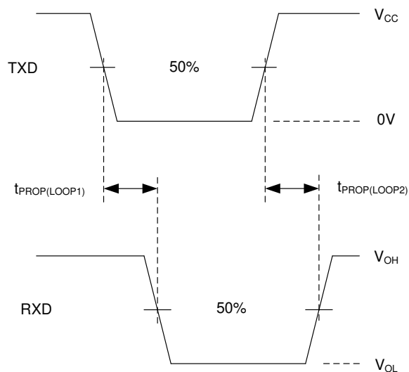
图 7-6. t_{\text{PROP(LOOP)}} Test Circuit and Measurement
