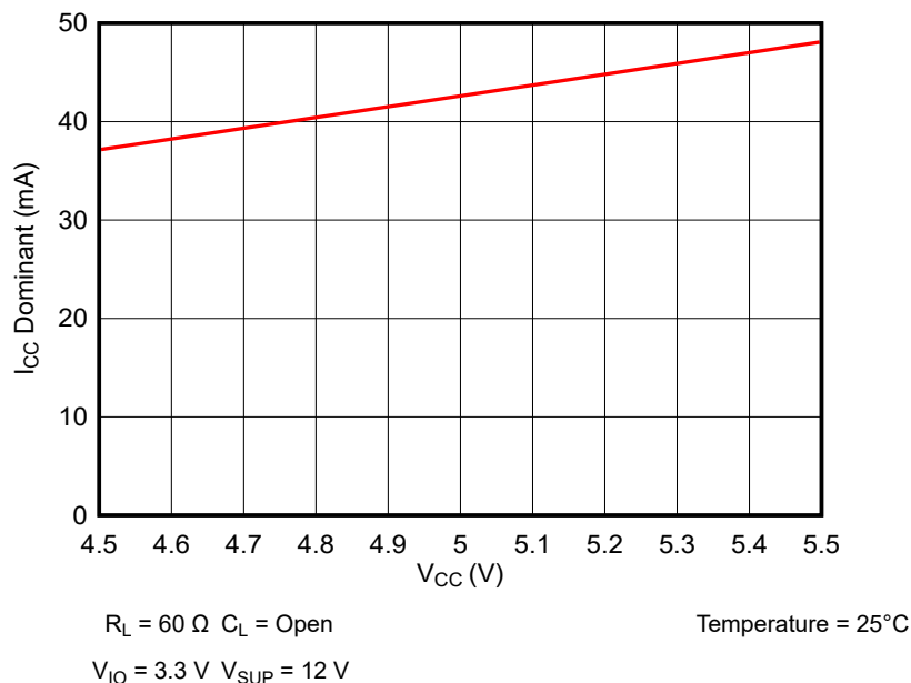
图 9-3. I_{CC} Dominant over I_{CC} Supply Voltage
