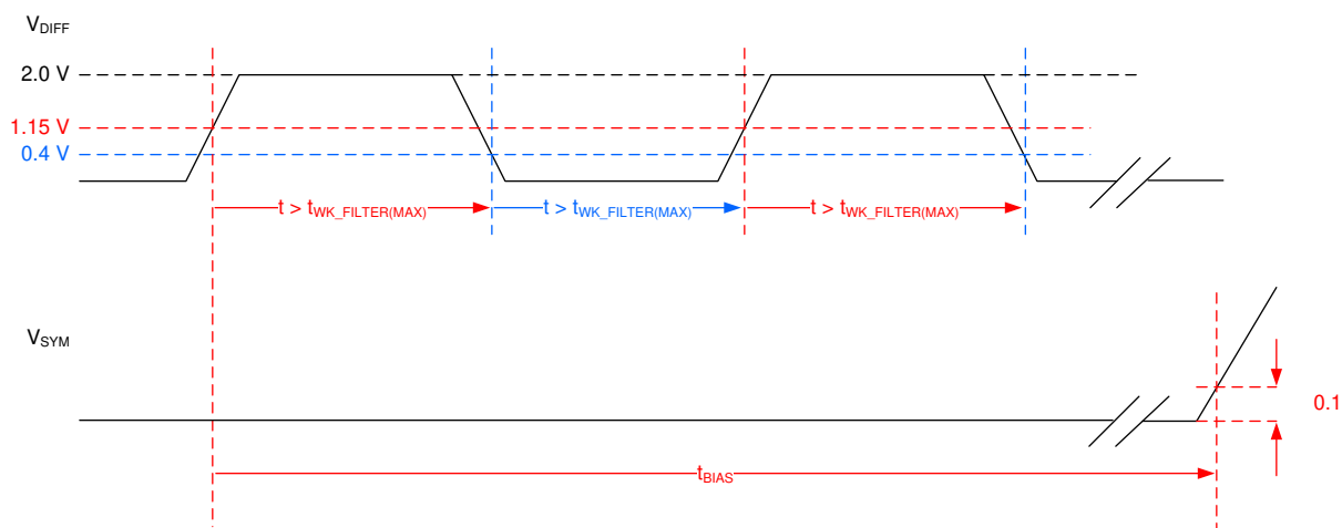
图 7-9. Bias Reaction Time Measurement
