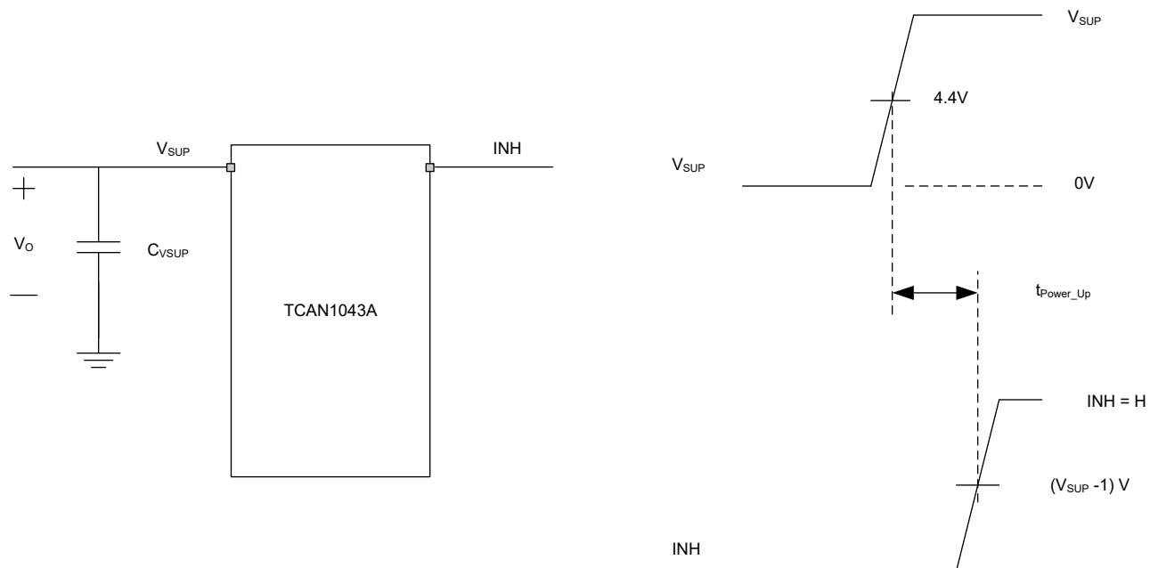
图 7-10. Power-Up Timing
