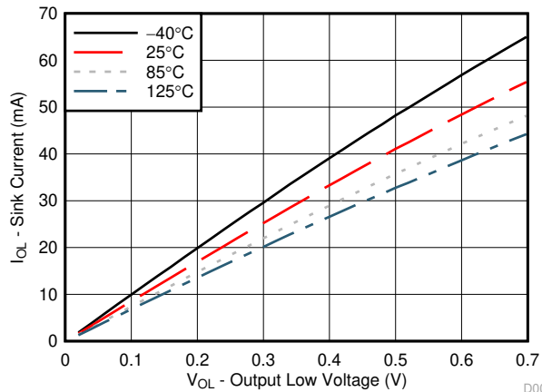
图 6-7. I/O Sink Current vs Output Low Voltage for Different Temperature ( T_A ) for V_{CC} = 3.3\text{ V}
