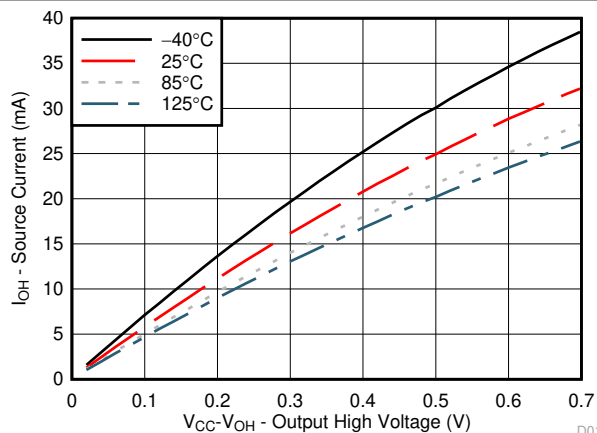
图 6-11. I/O Source Current vs Output High Voltage for Different Temperature ( T_A ) for V_{CC} = 2.5\text{ V}
