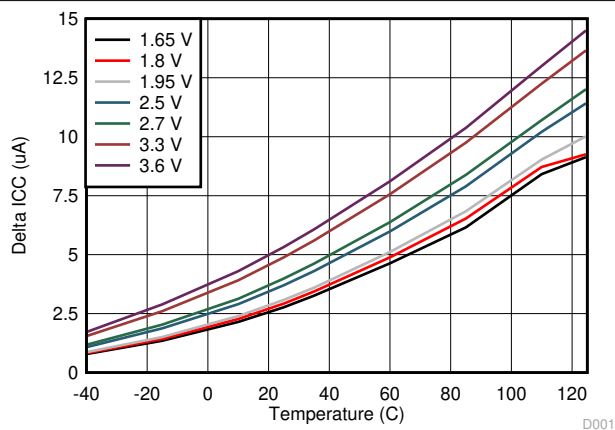
图 6-14. \Delta I_{CC} vs Temperature for Different V_{CC} ( V_I = V_{CC} - 0.6 V)
