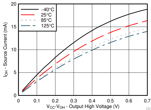
图 6-9. I/O Source Current vs Output High Voltage for Different Temperature ( T_A ) for V_{CC} = 1.65\text{ V}
