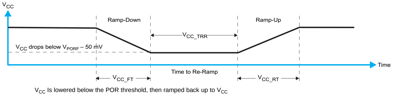
Figure 40. Voltage Waveform for Power-On Reset
